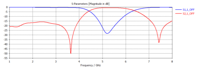
Fig. 8 S-parameters of the BPF at case 2.
