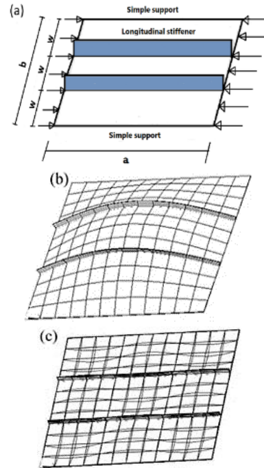
Fig. 2 Buckling mode shapes for \alpha = 3 , n = 2 , (a) boundary condition and loading, (b) Symmetric configuration, (c) Anti-symmetric configuration.
