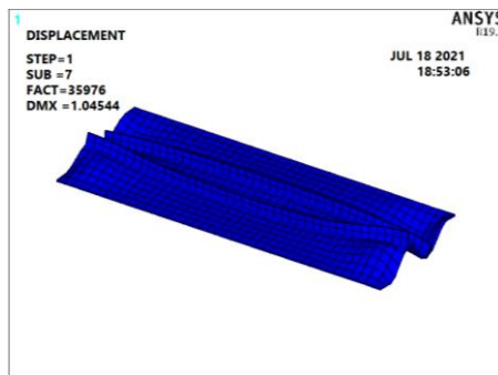
Critical buckling load for compression plate with two stiffeners of flat-bar section.
