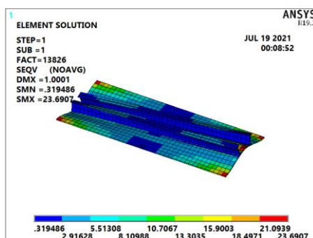
First buckling load for compression plate with two stiffeners of WT12 x 27.5 section.
