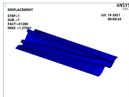
Critical buckling load for compression plate with two stiffener of ST 9 x 35 section.
