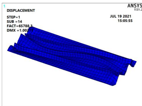
Critical buckling load for compression plate with \alpha = 10 .
