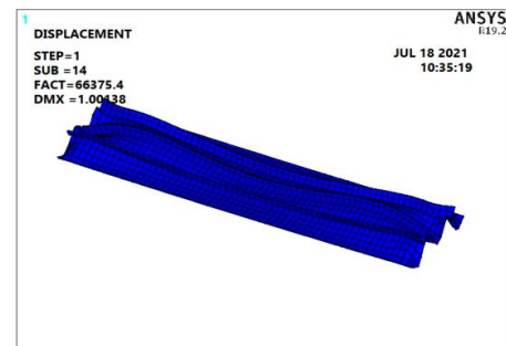
Critical buckling load for compression plate with \alpha = 15 .
