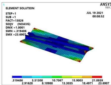
First buckling load for compression plate with two stiffener of ST 9 x 35 section.
