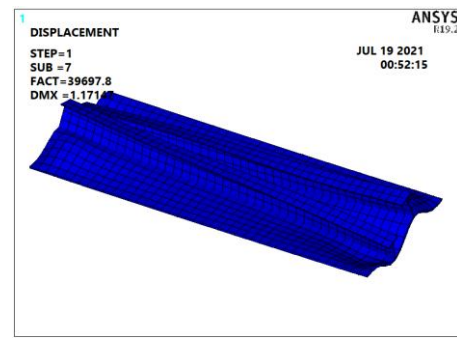
Critical buckling load for compression plate with two stiffeners of WT 12 x 27.5 section.
