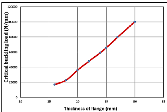
Fig. 8 Critical buckling load versus flange thickness.
