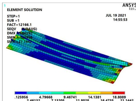
First buckling load for compression plate with \alpha = 12.5 .
