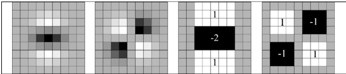
Figure 2: Discretization of second Order Gaussian Kernels
