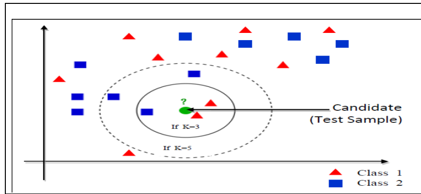
Figure (5): An example of KNN Technique in classification
