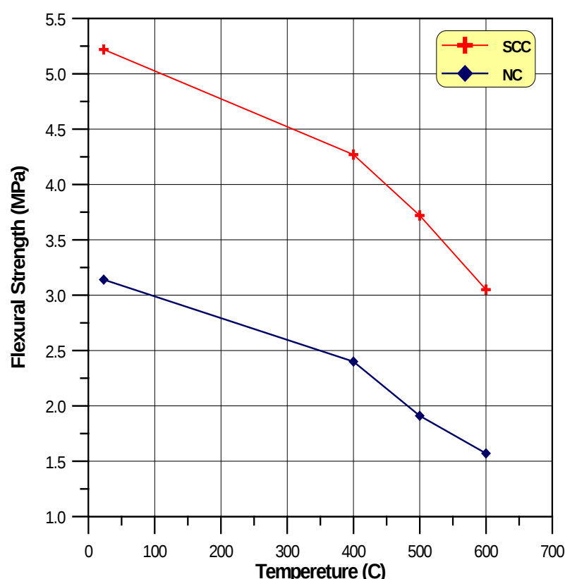
Figure (3): Relationship between flexural strength and firing temperture.
