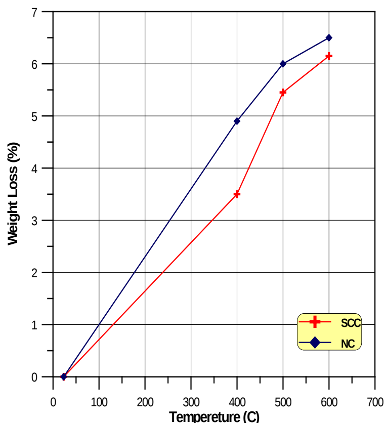
Figure (5): Relationship between weight loss and firing temperture for cubes.
