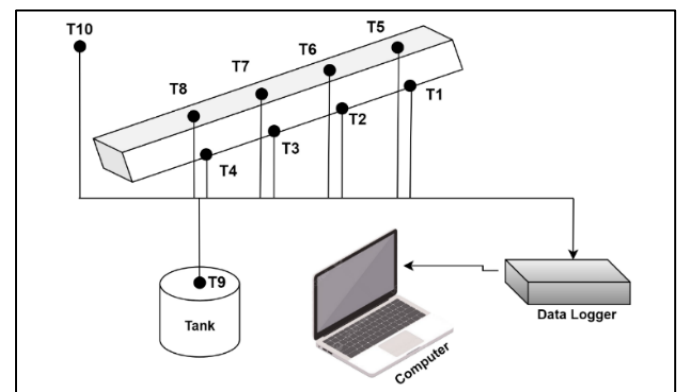
Fig. 7 Thermocouples location.
