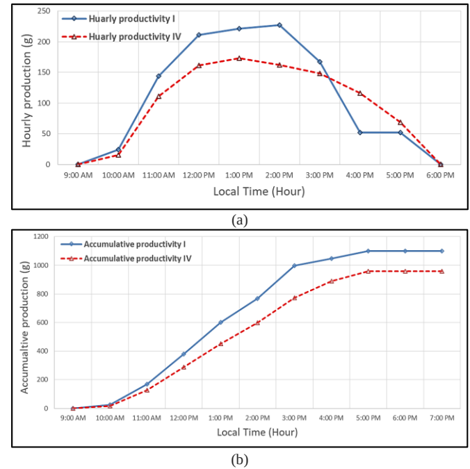
Fig. 22 (a) Hourly productivity. (b) Daily productivity for systems (I) and (IV).
