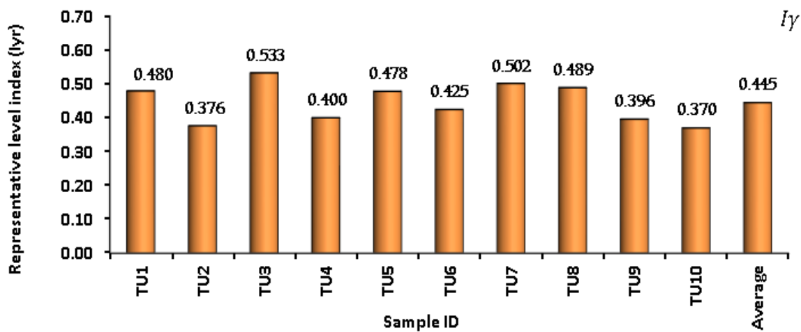
Fig. 7: Show values of gamma representative level index ( I_\gamma ) for all samples
