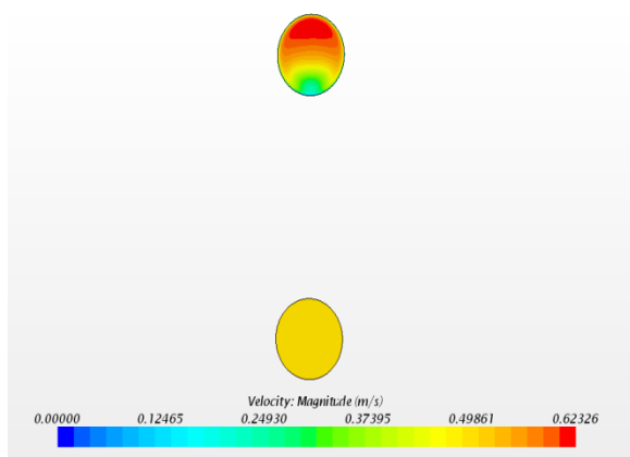
Fig. 30. Inlet and outlet faces velocity magnitude in turbulent flow
