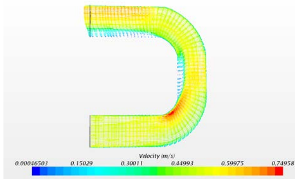
Fig. 26. Velocity magnitude for turbulent flow
