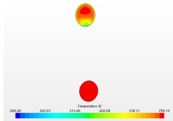
Fig. 31. Inlet and outlet faces temperature distribution in turbulent flow
