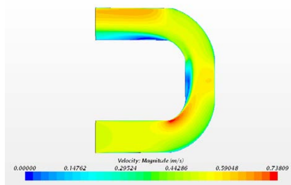
Fig. 29. Inlet and outlet face velocity vector in turbulent flow
