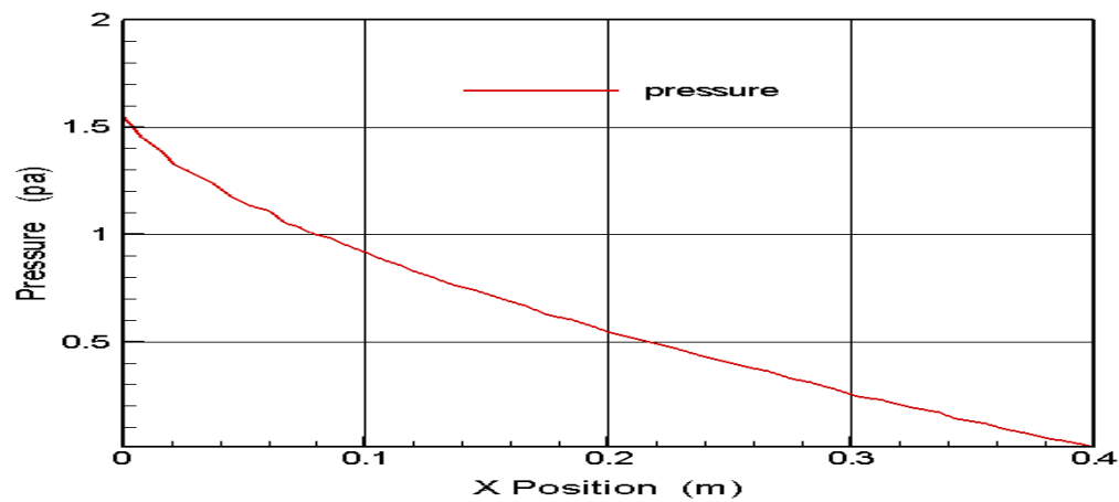
Fig. 12. Centre line pressure distribution in laminar flow
