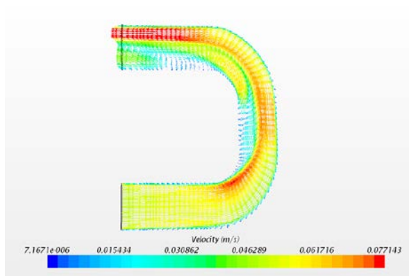
Fig. 22. Velocity vector for laminar flow
