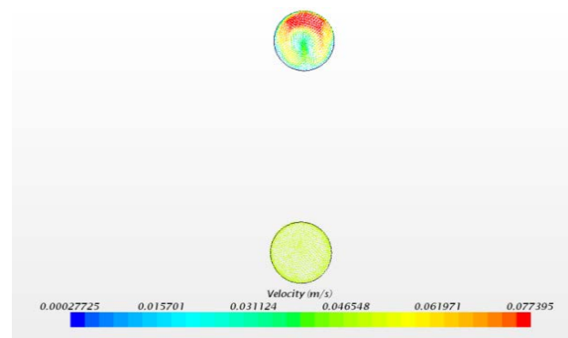
Fig. 23. Inlet and outlet face velocity vector in laminar flow
