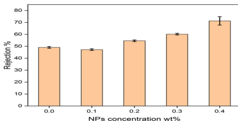
Figure 3: Effects of WO 2.89 loading on membrane rejection efficiency against tinzaparin sodium
