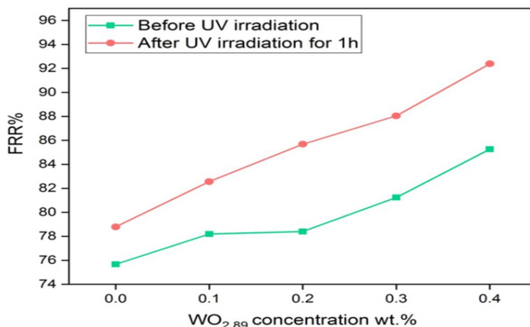
Figure 4: FRR of the neat and modified membranes with and without UV light irradiation
