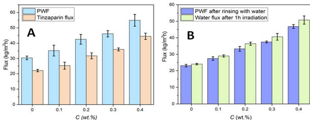
Figure 2: Flux values of neat and modified membranes at different processes; A- Flux with tinzaparin solution in the feed; B- Water flux before/after UV irradiation
