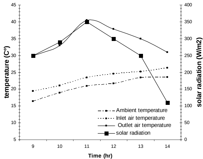
Fig.3. air ambient temperature, air inside, outside of the collector solar and solar radiation for angle 30^\circ . (history 21/11/2008)
