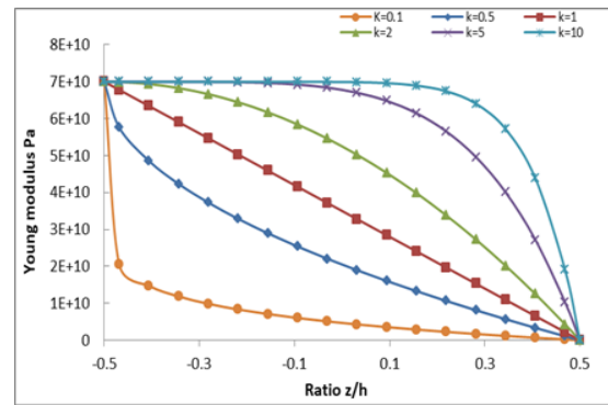
Figure 2: Young modulus versus thickness
