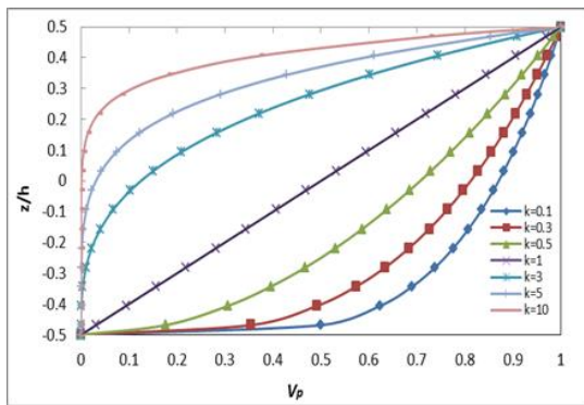
Figure 1: Volume fraction versus thickness
