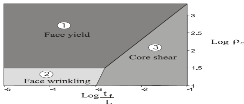
Figure 3: Three-point bending failure mode map for a sandwich beam having aluminium skins and FG core [36]
