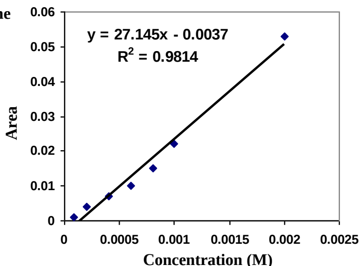
Fig. (15): The calibration curve between the integrated area under the peak measured at different concentration in ethanol at \lambda = (228 - 246)\text{nm} of L_1\text{Ni} complex solution.
