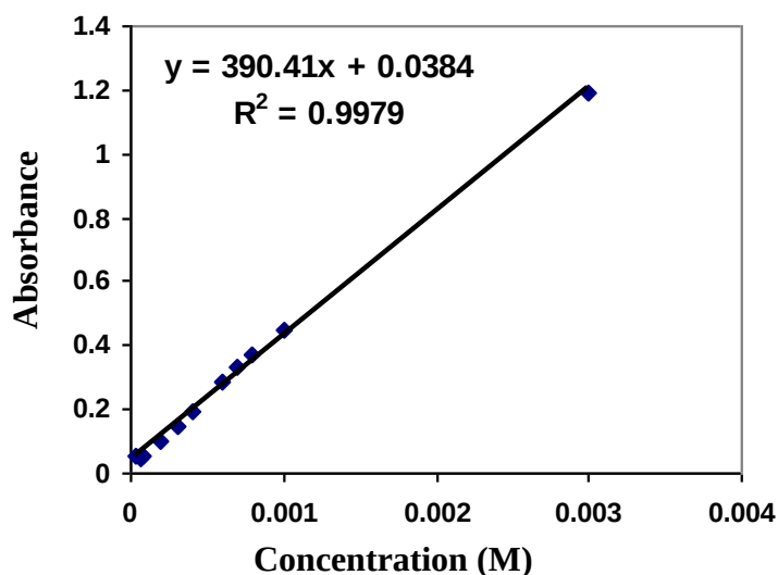
Fig. (12): The zero -order calibration curve of L_2Ni complex solution at different concentration at \lambda = 240 \text{ nm}
