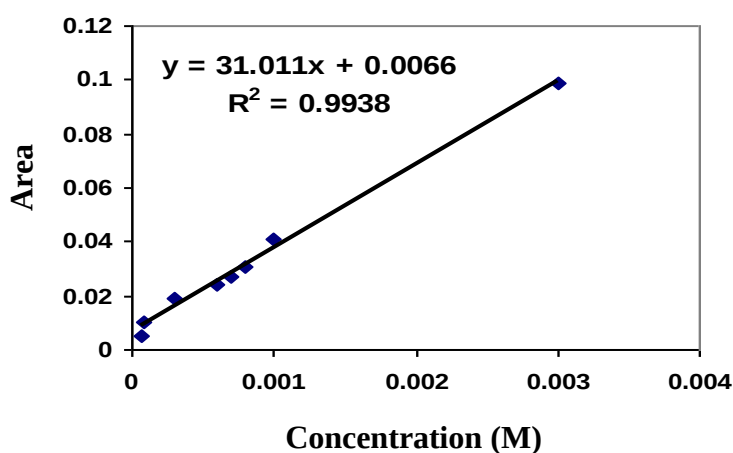
Fig. (16): The calibration curve between the integrated area under the peak measured at different concentration in ethanol at \lambda = (230 - 250)\text{nm} of L_2\text{Ni} complex solution.
