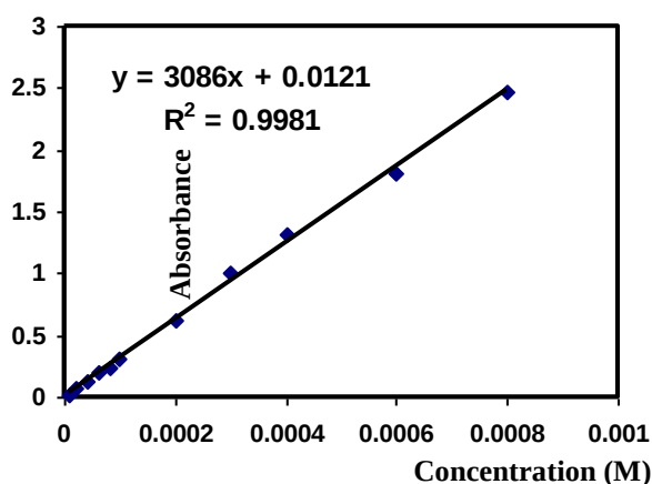
Fig. (4): The zero -order calibration curve of L_2Co complex solution at different concentration at \lambda = 278 nm
