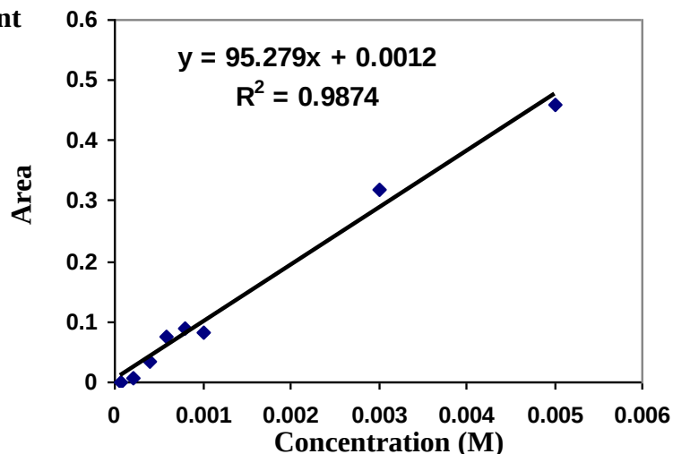
Fig. (13): The calibration curve between the integrated area under the peak measured at different concentration in ethanol at \lambda = (236 - 264)\text{nm} of \text{L}_1\text{Ni} complex solution.
