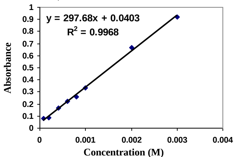
Fig. (10): The zero -order calibration curve of L_1Ni complex solution at different concentration at \lambda = 234 nm
