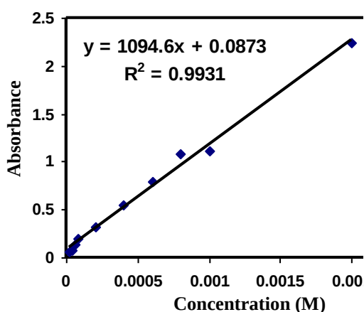
Fig. (3): The zero -order calibration curve of L_1Co complex solution at different concentration at \lambda = 276 nm
