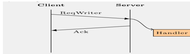
Figure 3. Asynchronous Protocol
