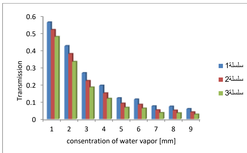
Fig.(4)Effect of water vapor on 5μm IR transmission at different Distance (series1 700m, Series2 800m, series3 900m)
