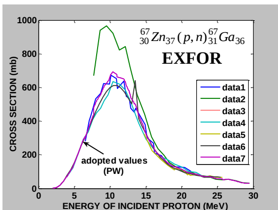
Figure (5): The adopted cross section of the ^{67}_{30}\text{Zn}_{37} target element (present work) compared with EXFOR Library. Data 1:Ref. No.[15]; Data 2:Ref. No.[12]; Data 3:Ref. No.[17]; Data 4:Ref. No.[18]; Data 5:Ref. No.[19]; Data 6:Ref. No.[19]; Data 7: (PW)
