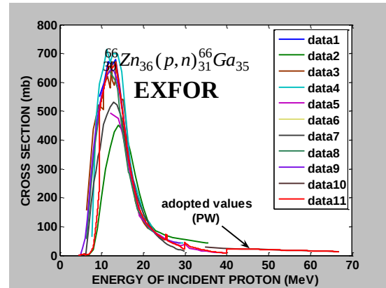
Figure (2): The adopted cross section of the ^{66}_{30}\text{Zn}_{36} target element (present work) compared with EXFOR Library. Data 1:Ref. No.[13]; Data 2:Ref. No.[14]; Data 3:Ref. No.[15]; Data 4:Ref. No.[12]; Data 5:Ref. No.[16]; Data 6:Ref. No.[17]; Data 7:Ref. No.[18]; Data 8:Ref. No.[19]; Data 9:Ref. No.[19]; Data 10:Ref. No.[20]; Data 11: (PW).
