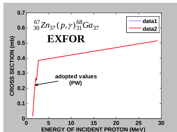
Figure (6): The adopted cross section of the ^{67}_{30}\text{Zn}_{37} target element (present work) compared with EXFOR Library. Data 1:Ref. No.[9]; Data 2: (PW).
