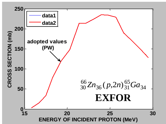
Figure (3): The adopted cross section of the ^{66}_{30}\text{Zn}_{36} target element (present work) compared with EXFOR Library. Data 1:Ref. No.[12]; Data 2: (PW).
