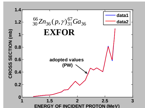
Figure (4): The adopted cross section of the ^{66}_{30}\text{Zn}_{36} target element (present work) compared with EXFOR Library. Data 1:Ref. No.[10]; Data 2: (PW).
