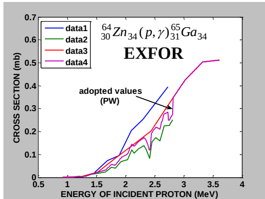
Figure (1): The adopted cross section of the ^{64}_{30}\text{Zn}_{34} target element (present work) compared with EXFOR Library. Data 1:Ref. No.[9]; Data 2:Ref. No.[10]; Data 3:Ref.
