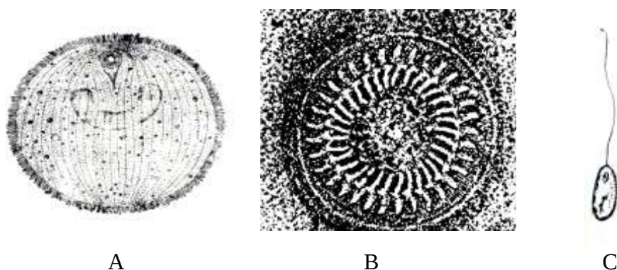
Fig (1): Three type of primary animal that are: (A) Ichthyophthirius multifiliis (B) Trichodina cottidarum (C) Plisthophora typicalis
