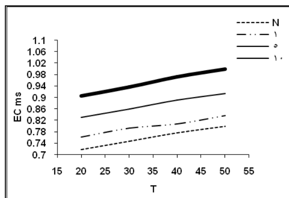
Fig. (2): The effect of 450 gauss static magnetic field on electrical conductivity of 1000 ppm \text{CaCl}_2 \cdot 2\text{H}_2\text{O} solution at pH 7.2.
