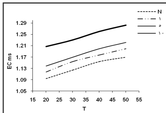
Fig. (8): The effect of 450 gauss static magnetic field electrical conductivity of 1000 ppm \text{CaCl}_2 \cdot 2\text{H}_2\text{O} at solution at pH 7.8.
