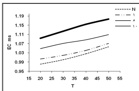
Fig. (6): The effect of 450 gauss static magnetic field on the electrical conductivity of 1000 ppm solution at pH 7.6.
