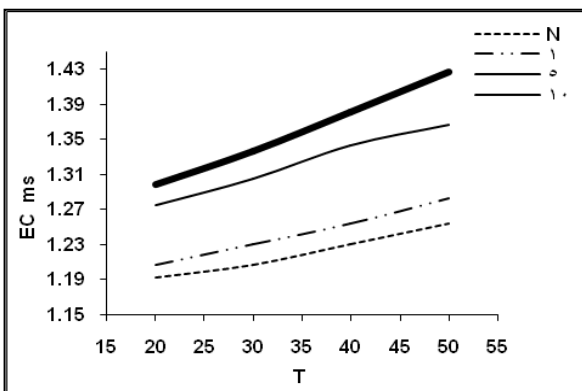
Fig. (10): The effect of 450 gauss static magnetic field electrical conductivity of 1000 ppm solution at pH 8.0.
