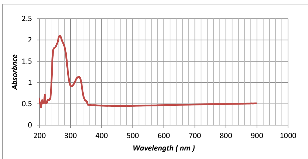
Fig(5):UV-visible absorption spectrum of ZnO Nanoparticles.
