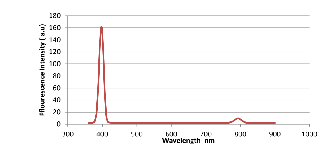
Fig.(7):fluorescence intensity as a function of wavelengths of ZnO nanoparticles
