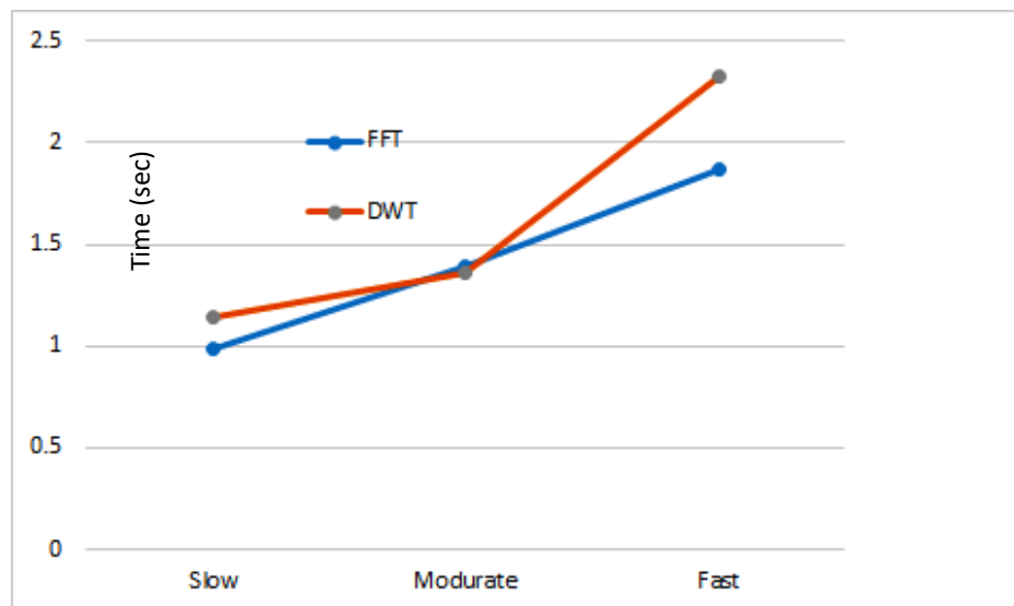
Fig (8). The computation time for applying Fourier and Walsh transform
