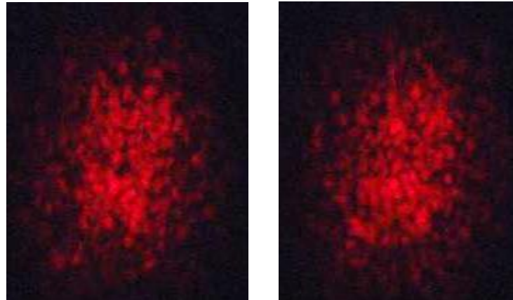
Fig (5). The change in the speckle pattern due to applying the vibration on the fiber
