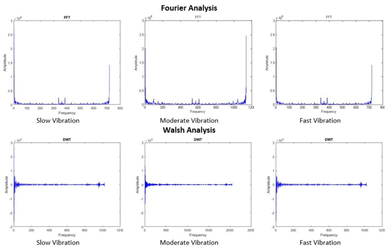
Fig (6). The Fourier (magnitude) and Walsh coefficients of the speckle pattern differences
