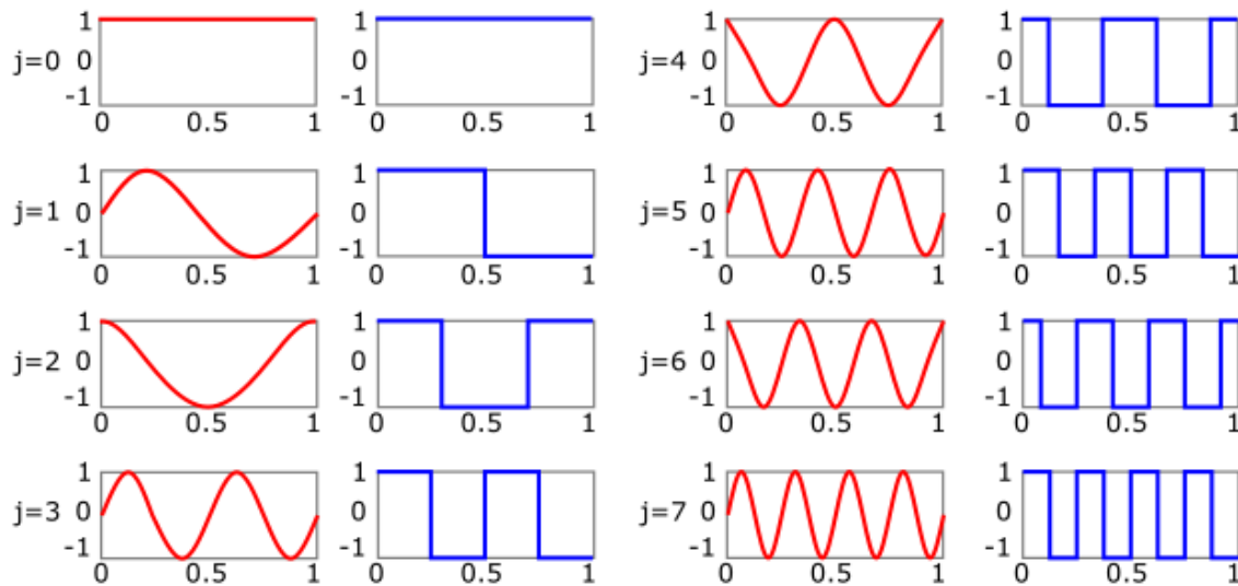
Fig (2). The Fourier (in red) and equivalents Walsh (in blue) transforms
