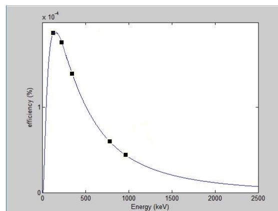
Fig (4) Eu-152 efficiency curve for the case \pm 0.5\sigma .
