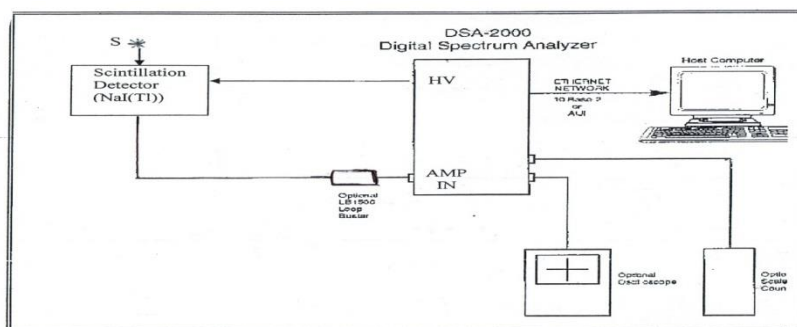
Fig (2) NaI(Tl) detector system
