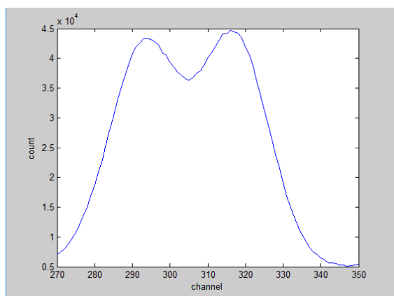
Fig (5) Part of spectrum of two energies 609 and 661 keV of Ra-226 and Cs-137 sources brought together.
