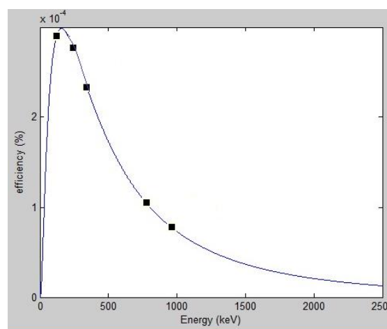
Fig (3) Eu-152 efficiency curve for the case \pm\sigma
