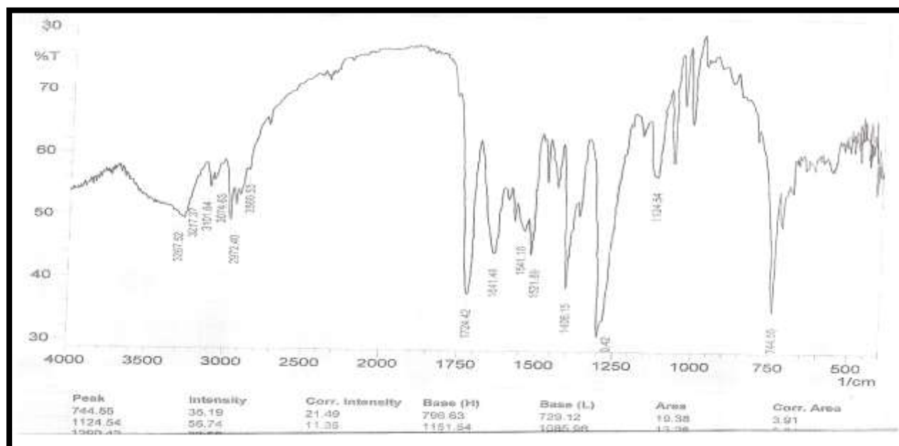
Fig-3:- IR spectrum of the ligand [\text{H}_2\text{L}]
