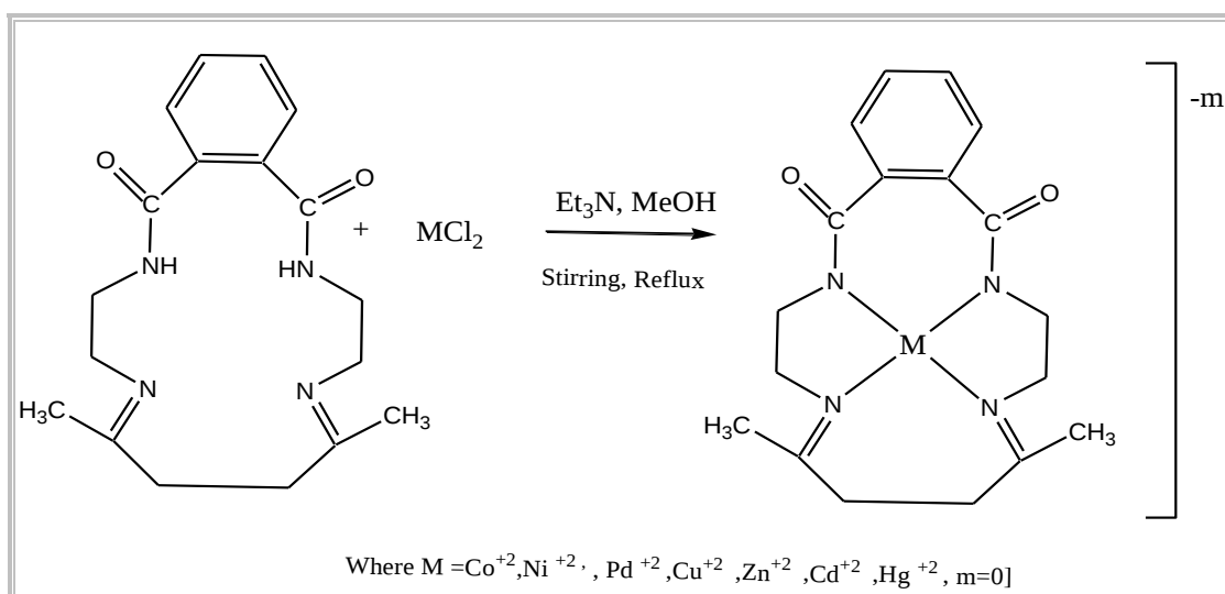
Scheme (3): Preparation of [C 2 , C 3 , C 4 , C 6 , C 7 , C 8 ] complexes
