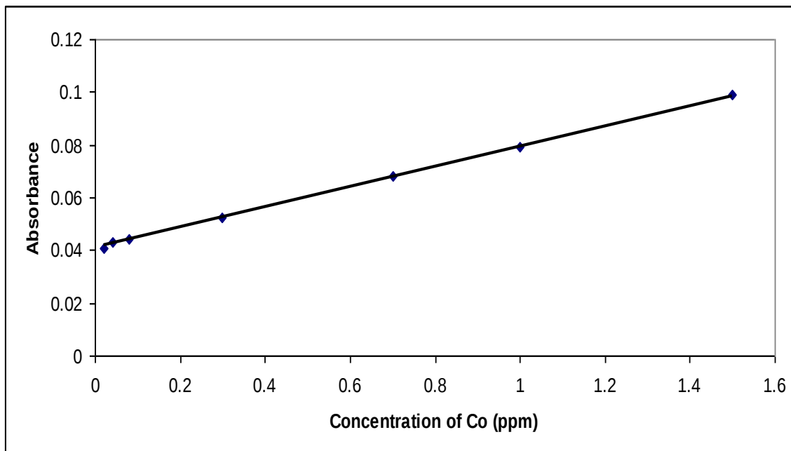
Figure (11) calibration curve of \text{Co}^{2+} ion.
