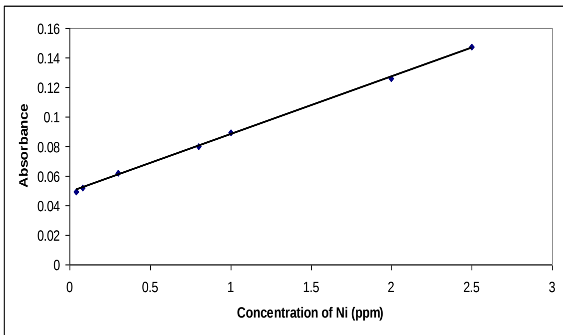
Figure (12) calibration curve of \text{Ni}^{2+} ion.
