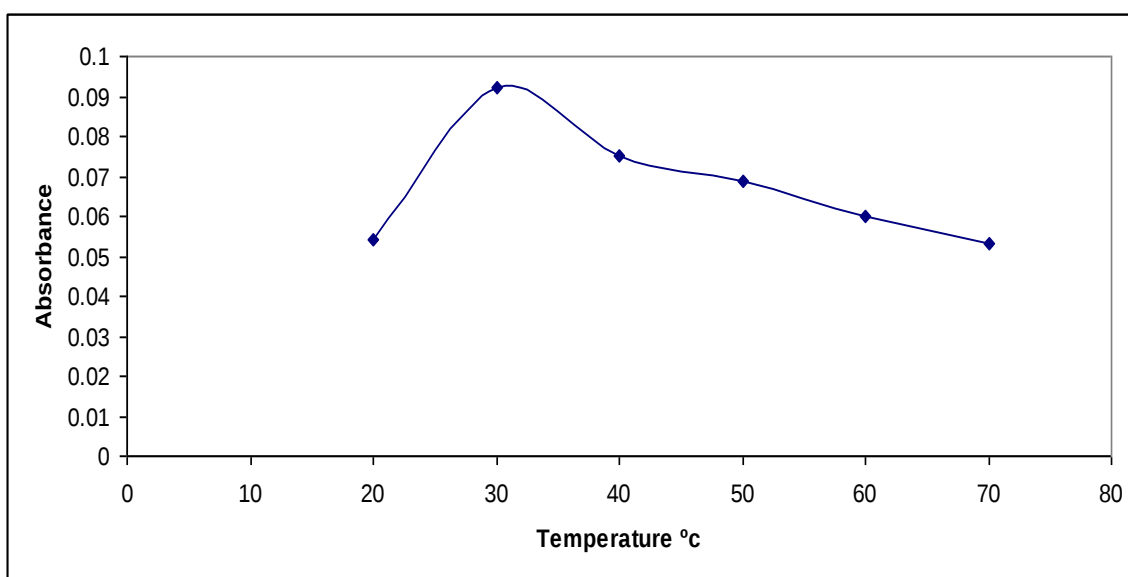
Fig.(4) Effect of temperature on the absorbance of Ni-MBTAMP complex.
