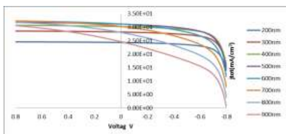
Fig.1: I-V characteristic of (ZnSe/MASnI 3 /CuSCN) cell the
