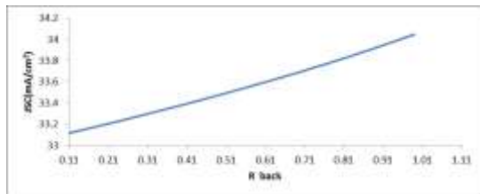
Fig (8) Effect of reflective cell concentration (n- ZnSe / p-MASnI3 / p-CuSCN) on J_{sc}
