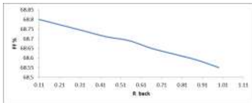
Fig (10) Effect of reflective cell concentration (n- ZnSe / p-MASnI3 / p-CuSCN) on FF
