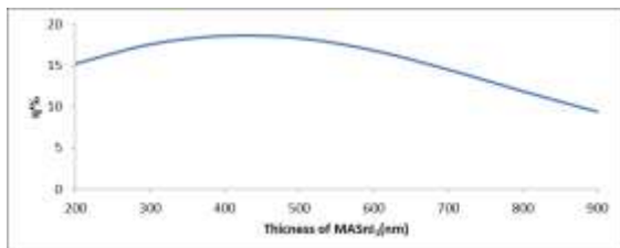
Fig (5) Effect of thickness on the absorber layer p-MASnI3 on the efficiency of the cell
