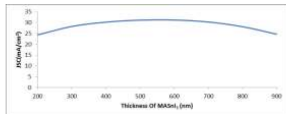
Fig. 2: Effect of thickness of the absorbent layer p-MASnI 3 on J_{sc}
