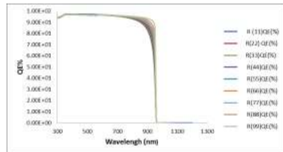
Fig (12) Effect of reflective cell concentration (n- ZnSe / p-MASnI3 / p-CuSCN) on QE
