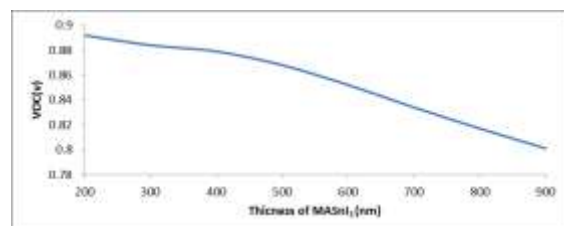
Fig. 3: Effect of thickness of the absorbent layer p-MASnI 3 on V_{oc}
