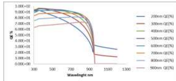
Fig(6) QE with wavelength at different thickness variation
