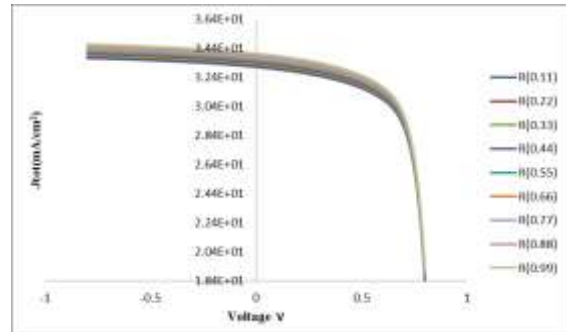
Fig (7) (I-V) characteristic of the n- ZnSe/p-MASnI3/p-CuSCN cell with different reflectivity
