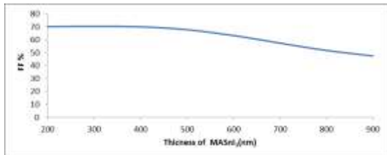
Fig. 4: The effect of thickness of the absorber layer p-MASnI3 on FF
