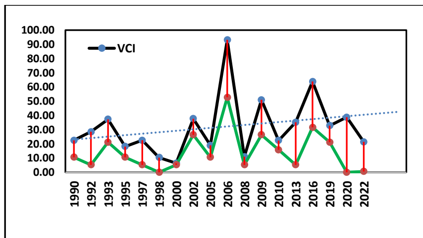
Figure 6. Time series of VCI for monitoring Drought and Desertification.
