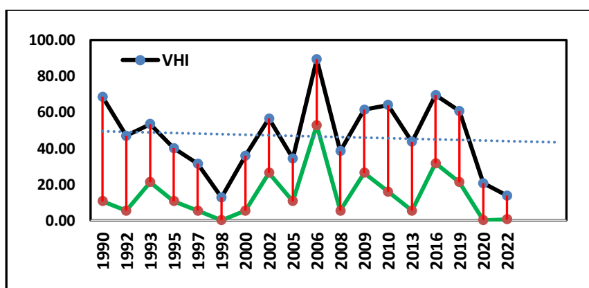
Figure 8. Time series of VHI for monitoring Drought and Desertification.
