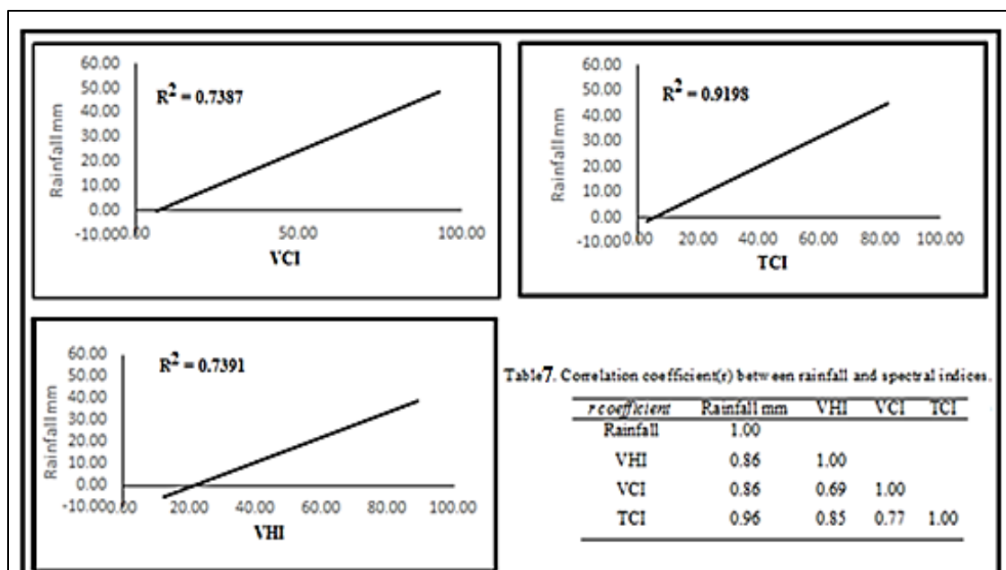
Figure 9. The regression coefficient R^2 between Rainfall and indices.
