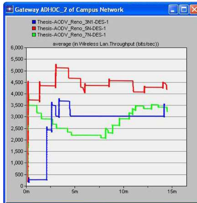
Figure 12 Average Throughput (bits/sec) Comparison between 3, 5, 7 Mobile Nodes in Reno TCP Variant
