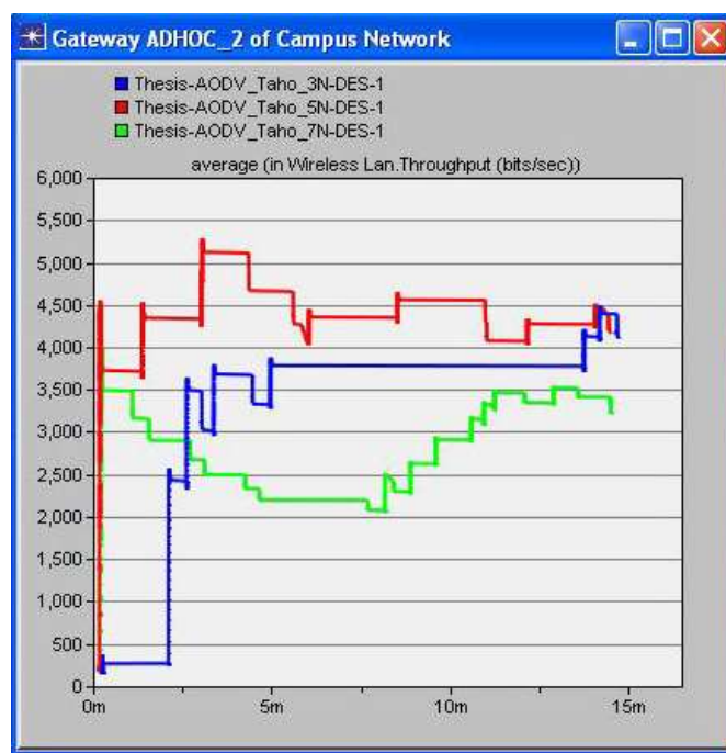
Figure 10 Average Throughput (bits/sec) Comparison between 3, 5, 7 Mobile Nodes in Tahoe TCP Variant
