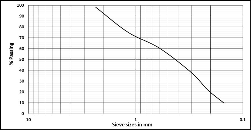
Figure 2: Grading curve of River sand
