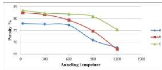
Fig. 6: variation Porosity as a function of different annealing temperatures for compounds A, B and C
