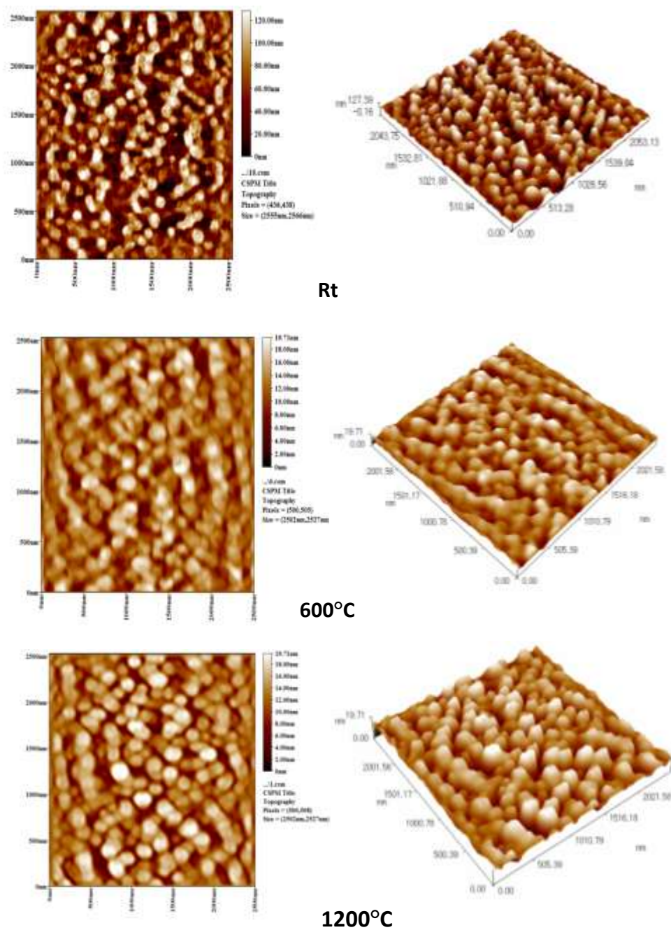
Fig. 9. AFM images of B in (2D-3D) dimensional
