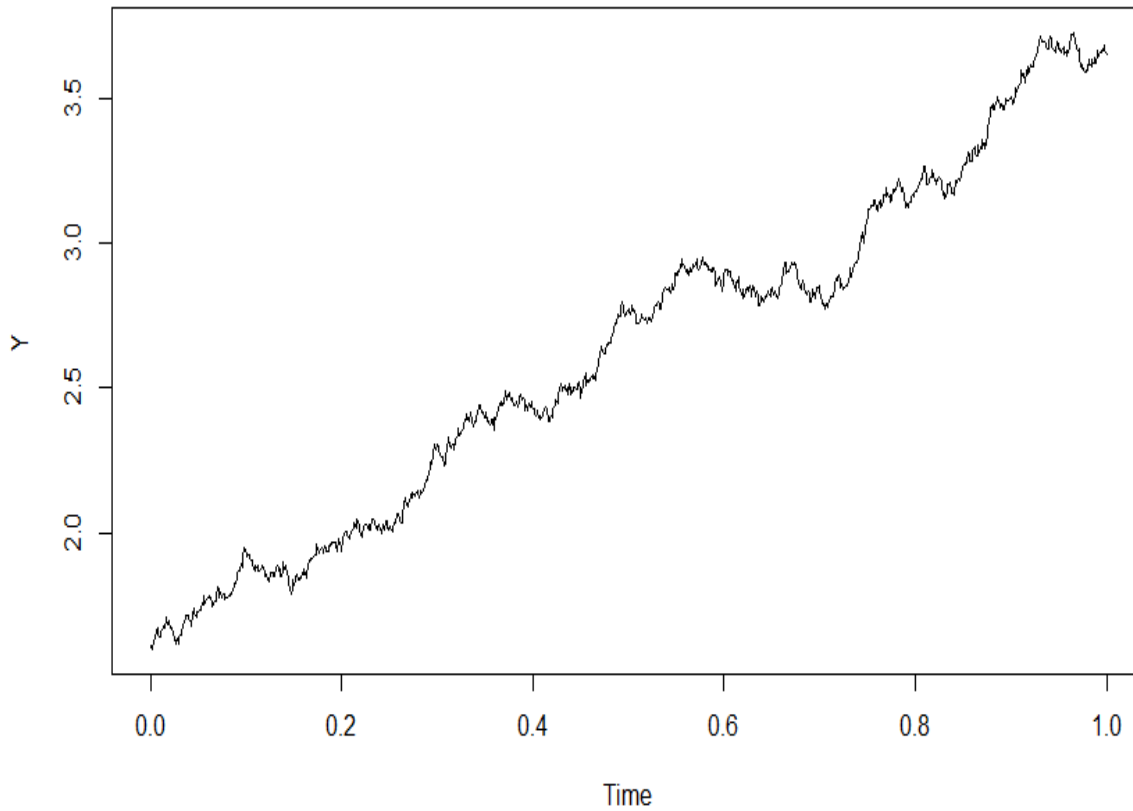
Figure 2: Sample path for SDDE in drift term
