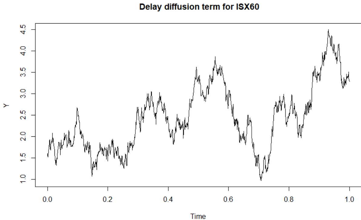
Figure 3: Sample path for SDDE in diffusion term
