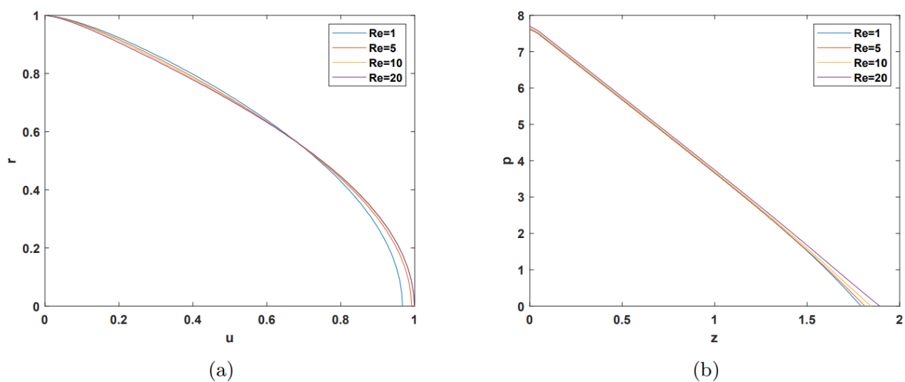
Figure 3: Effect Re on (a) Velocity and (b) Pressure.
