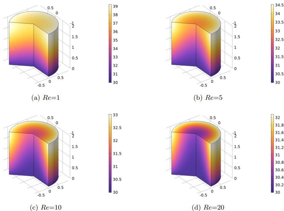
Figure 6: Effect Re on 3D Temperature field.
