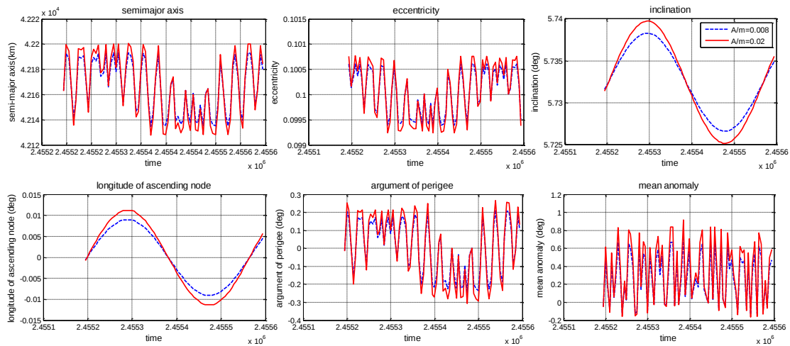
Figure (5.10) the perturbation due to solar radiation pressure in one year at different A/m ratio. ( a = 42164\text{km} , e = 0.1 , \Omega = 0 )
