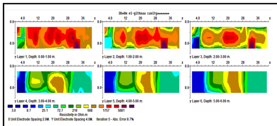
Figure (4) Inversion model for Um El-Githoaa cavity shows horizontal slices of the 3D resistivity distribution with depth. The highest resistivity anomaly more than (800 \Omega m) is related to subsurface cavity using robust constrain method.
