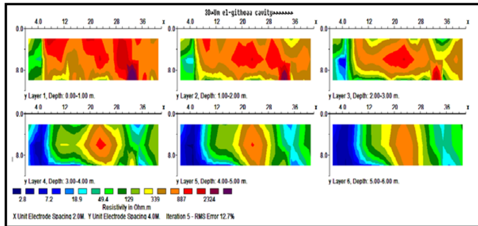
Figure (3) Inversion model for Um El-Githoaa cavity shows horizontal slices of the 3D resistivity distribution with depth. The highest resistivity anomaly more than (800 \Omega m) is related to subsurface cavity using standard Least-square method.
