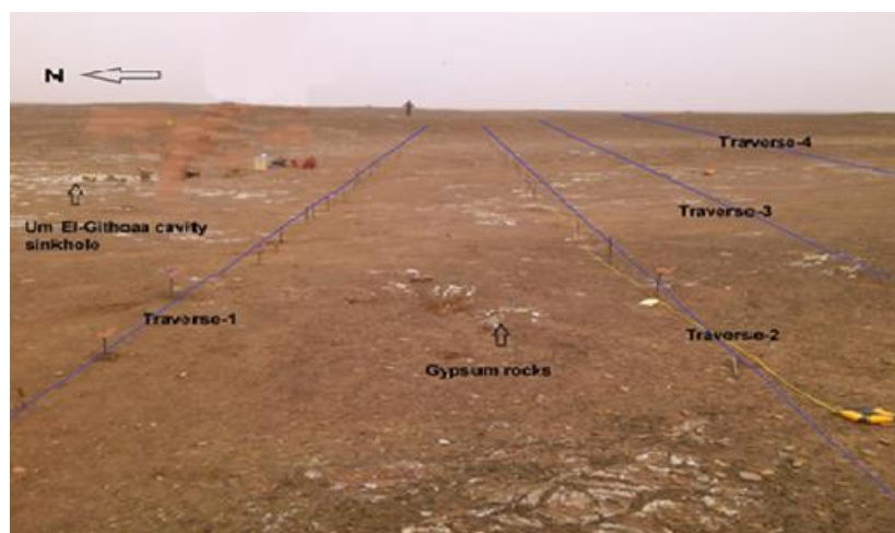
Figure (2) 2D Dipole-dipole traverses above Um El-Githoaa cavity.
