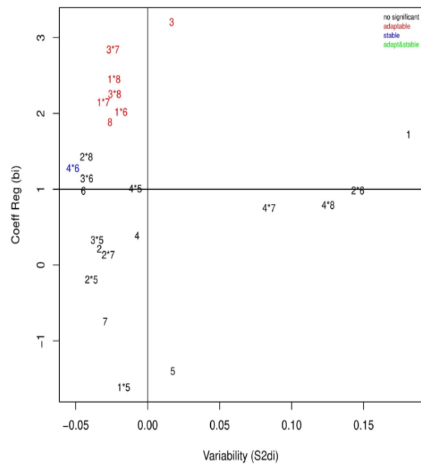
Figure 2. Stability and adaptability analysis for ear width
