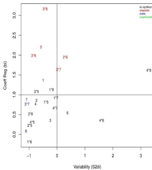
Figure 9: Stability and adaptability analysis for biological yield.
