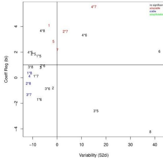
Figure 6. Stability and adaptability analysis for weight of kernel ear -1
