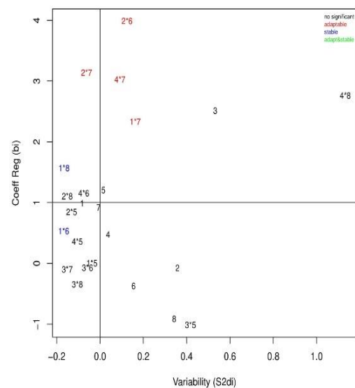
Figure 10: Stability and adaptability analysis for kernel
