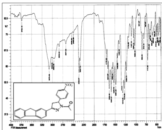
Fig.(1): FT-IR spectrum for compound (2a)
