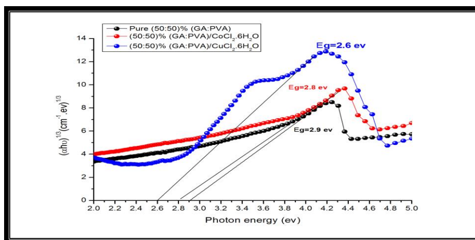
Figure 5. Relation between (\alpha h\nu)^{1/3} versus (h\nu) of (50:50)%GA/PVA doping By (\text{COCl}_2.6\text{H}_2\text{O}) & (\text{CuCl}_2.6\text{H}_2\text{O}) composite polymer.(direct forbidden energy)
