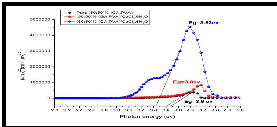
Figure 4. Relation between (\alpha h\nu)^2 versus (h\nu) of (50:50)%GA/PVA doping By (\text{COCl}_2.6\text{H}_2\text{O}) & (\text{CuCl}_2.6\text{H}_2\text{O}) composite polymer
