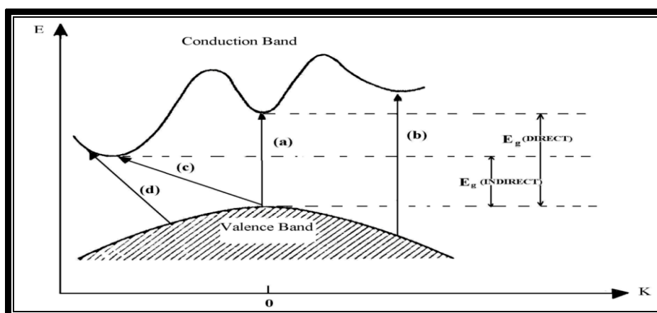
Figure1.The optical transitions(a)Allowed direct,(b)Forbidden direct; (c) Allowed indirect, (d) Forbidden indirect [5]
