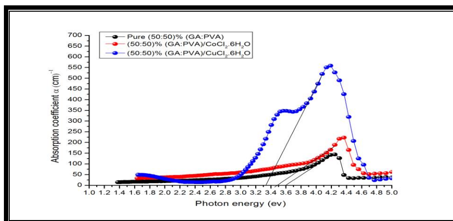
Figure 3. Relation between absorbance coefficient ( \alpha ) versus ( h\nu ) of (50:50)%GA/PVA doping By ( \text{CoCl}_2 \cdot 6\text{H}_2\text{O} ) & ( \text{CuCl}_2 \cdot 6\text{H}_2\text{O} ) composite polymer
