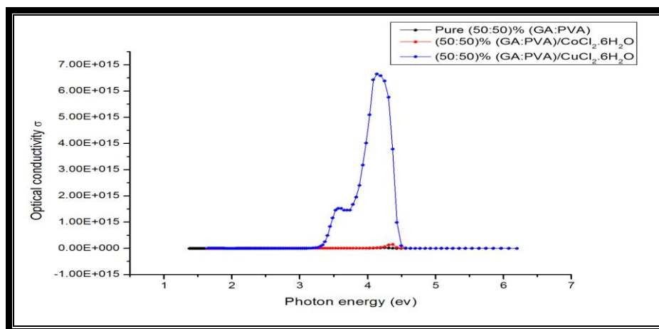
Figure 7. Optical conductivity of (50:50)%GA/PVA doping By (CoCl 2 .6H 2 O) & (CuCl 2 .6H 2 O).
