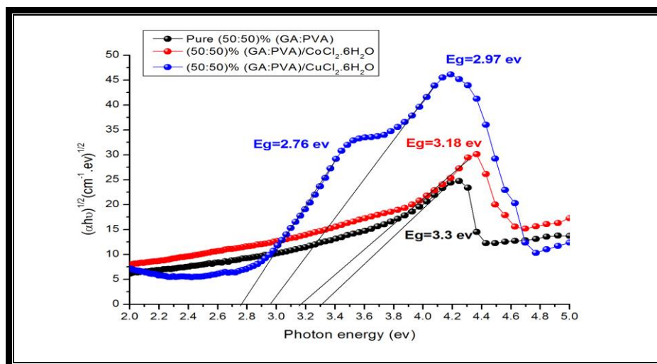
Figure 6. Relation between (\alpha h\nu)^{1/2} versus (h\nu) of (50:50)%GA/PVA doping By (\text{COCl}_2.6\text{H}_2\text{O}) & (\text{CuCl}_2.6\text{H}_2\text{O}) composite polymer.(indirect transitions)
