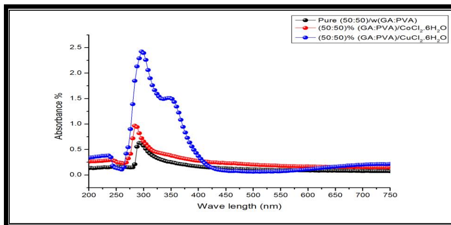
Figure2. The relationship between absorbance and the wave length of (50:50)%GA/PVA doping By ( \text{CoCl}_2 \cdot 6\text{H}_2\text{O} ) & ( \text{CuCl}_2 \cdot 6\text{H}_2\text{O} ) composite polymer
