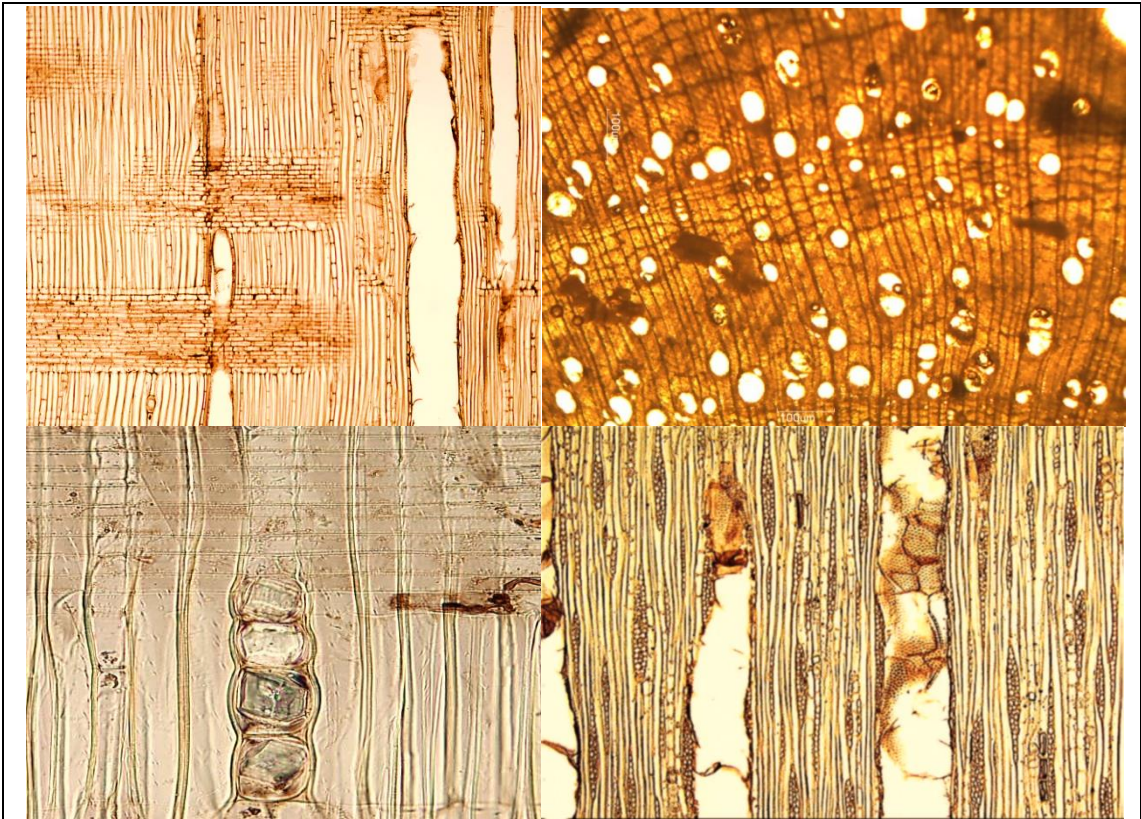
Figure (4) Wooden sections of the three faces (transverse, radial and tangential) with the presence of J. nigra crystals and tyloses.
