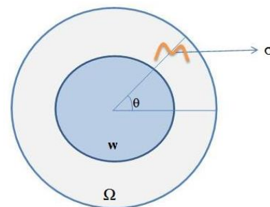
Figure 7: Disc domain, region \omega and location \sigma of internal filament sensor.
