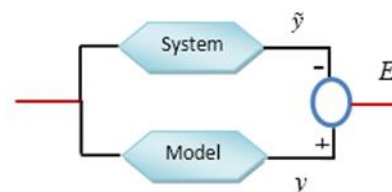
Figure 3.the observation error
