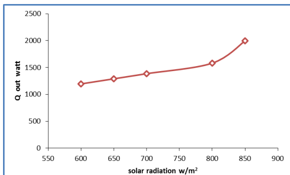
Figure (5) illustrate solar radiation variation with output energy.
