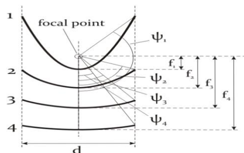
Figure (2) Relation between the focal length and the rim angle for a constant reflector diameter [16].
