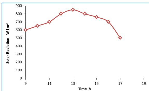
Figure (4) illustrate solar radiation variation with time .
