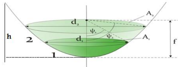
Figure (1) Geometrical dish parameters [16]
