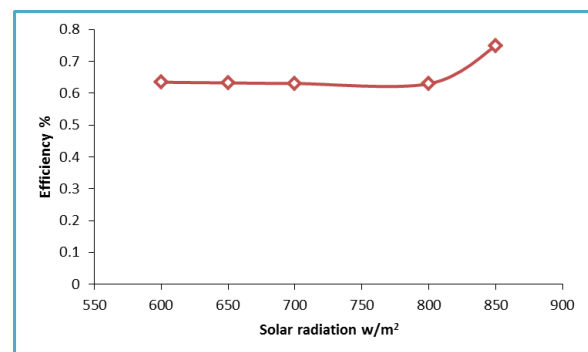
Figure (6) illustrate solar radiation variation with efficiency.
