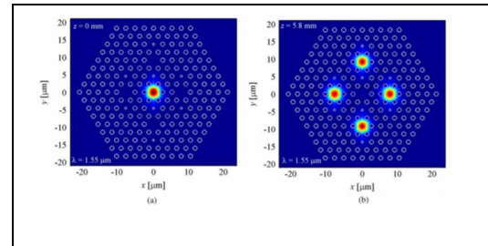
Fig. (3): Modal field distribution( x -component)of the multicore PCF( D/\Lambda=0.45, d/\Lambda=0.23 , and \Lambda=2.64\text{mm} )coupler (a) at z=0\text{ mm} , and (b) at z=5.8\text{ mm} at 1550nm wavelength [33].
