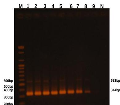
Fig (2): Ethidium bromide-stained agarose gel (1.5%) electrophoresis of DNA fragments generated by duplex PCR amplification of methicillin-resistance Staphylococcus aureus (MRSA) DNA dilutions. Lane (M): 100bp DNA ladder (promega), lanes (1-9): PCR product of femA gene (314bp) and mecA gene (533bp) using serial dilutions of DNA, Lane (N): PCR product of negative control (without DNA template).
