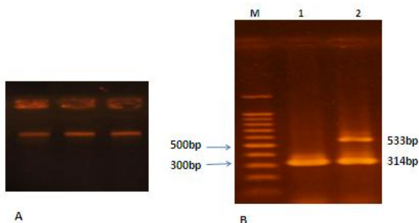
Fig (1): Ethidium bromide-stained agarose gel (1.5%) electrophoresis of: A) genomic DNA isolated from methicillin-resistance Staphylococcus aureus (MRSA) clinical isolates. B) DNA fragments generated by duplex PCR amplification of methicillin-resistance Staphylococcus aureus (MRSA). Lane (M): 100bp DNA ladder (promega), lanes (1-2): PCR product of femA gene (314bp) and mecA gene (533bp).
