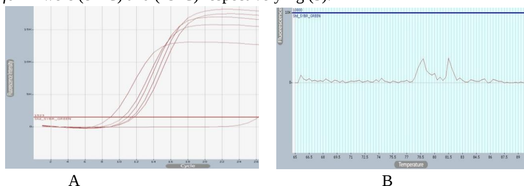
Fig (3): A) Fluorescent graph and B) melting curve analysis of mecA and femA genes amplified using SYBR Green real time PCR.
