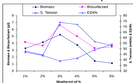
Fig (4): Effect of Weathered oil concentration on growth rate and biosurfactant production of Agrobacterium tumefaciens at 30 °C, pH 7 in shaker incubator at 150 rpm for 72 h
