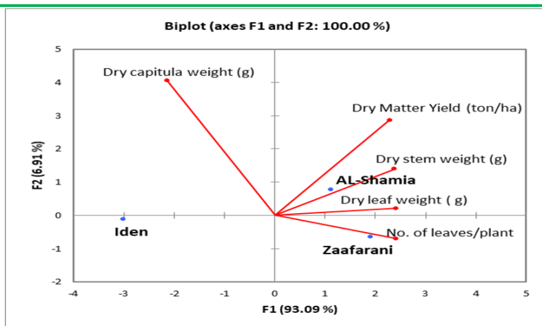
Figure 2. PCA plot showing the effect of safflower varieties on growth character at the average of both locations
