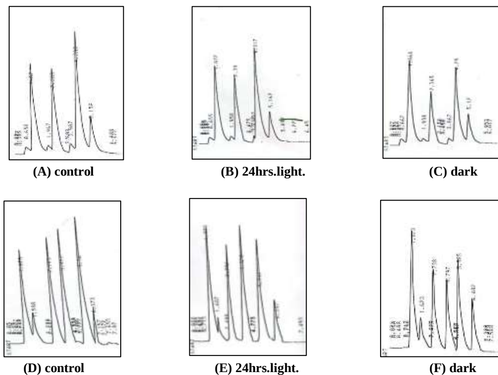
Figure (4): HPLC analysis of alkaloids (A,B ,C) and glycosides ( D, E, F ) in callus exposure to various period of light
