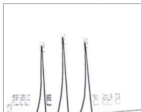
(B) glycosides
