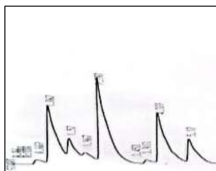
(A) Alkaloids
