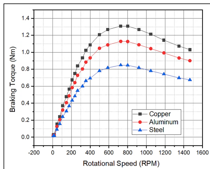
Figure 3: Braking torque with rotational speed
