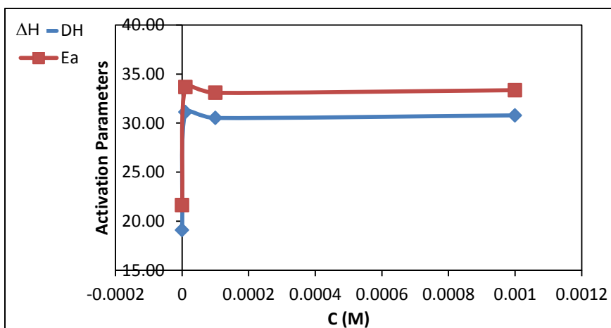
Figure 10: Variation of Ea and \Delta H versus concentration of azo dye in H 2 SO 4 solution
