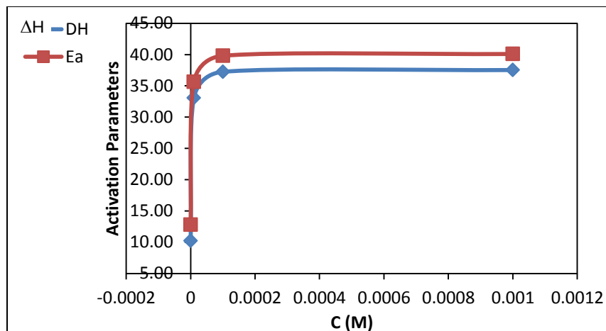
Figure 9: Variation of Ea and \Delta H versus concentration of azo dye in HCl solution
