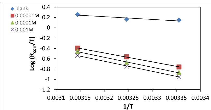
Figure 7: Arrhenius plots \log(R_{\text{corr}}/T) versus 1/T at different concentrations of azo dye in HCl
