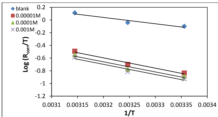
Figure 8 : Arrhenius plots \log(R_{\text{corr}}/T) versus 1/T at different concentrations of azo dye in \text{H}_2\text{SO}_4
