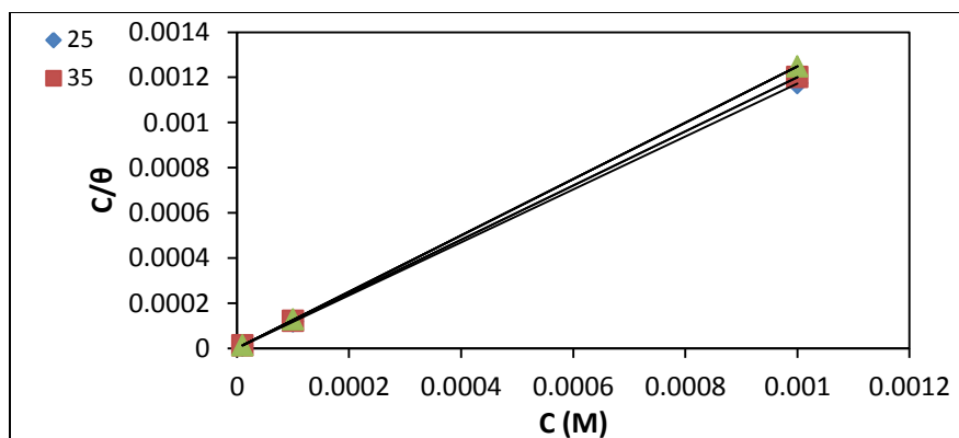
Figure 12: Langmuir adsorption isotherm of azo dye at different temperature in \text{H}_2\text{SO}_4 solution
