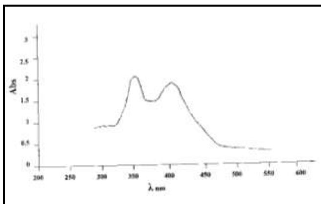
Figure 8: UV-Visiblespectra of Zn-complex (III) in DMF ( 1 \times 10^{-5} )
