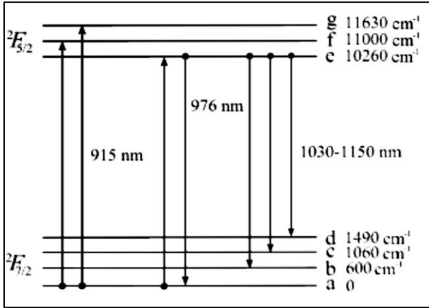
Figure(1): energy level diagram illustrating the ytterbium ground ^2F_{7/2} and excited ^2F_{5/2} state manifolds and possible transitions between the sub-levels [4].
