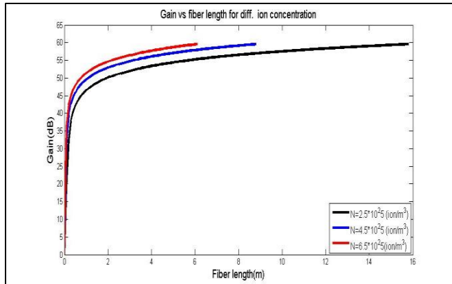
Figure (8): Gain vs fiber length at diff. ion concentration of (YDFA), p_p=25 mW, \lambda_p=968 nm, \lambda_s=1022 nm, a=2.5\mu\text{m} .
