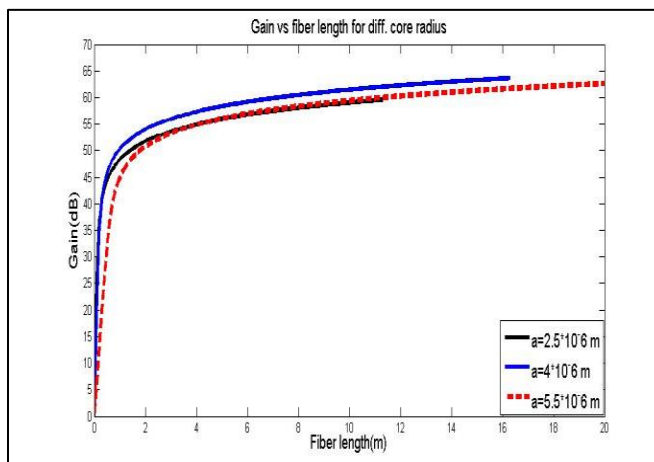
Figure (10): Gain vs. fiber length at diff. core radius of (YDFA), p_p=25 mW, \lambda_p=968 nm, \lambda_s=1022 nm, N=3.5 \times 10^{25} ion/m 3 .
