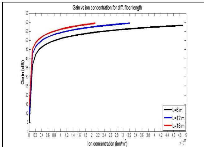
Figure (3): Gain vs. ion concentration at diff. fiber length of (YDFA), p_p=25\text{ mW} , \lambda_p=968\text{nm} , \lambda_s=1022\text{nm} , a=2.5\mu\text{m} .
