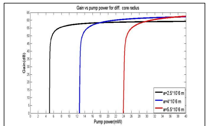
Figure (7): Gain vs. pump power at diff. core radius of (YDFA), L=10\text{m} , \lambda_p=968\text{nm} , \lambda_s=1022\text{nm} , N=3.5 \times 10^{25}\text{ ion/m}^3 .
