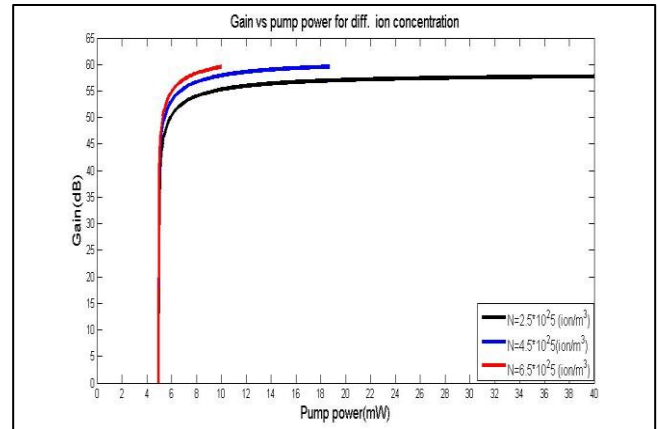
Figure (5): Gain vs. pump power at diff. ion concentration of (YDFA), L=10\text{m} , \lambda_p=968\text{nm} , \lambda_s=1022\text{nm} , a=2.5\mu\text{m} .
