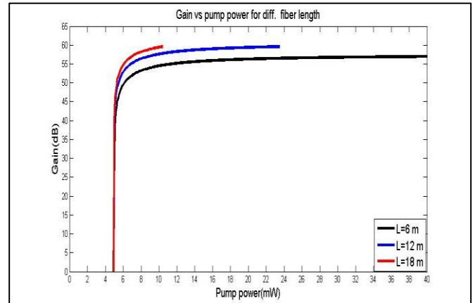
Figure (6): Gain vs. pump power at diff. fiber length of (YDFA), \lambda_p=968\text{nm} , \lambda_s=1022\text{nm} , a=2.5\mu\text{m} , N=3.5 \times 10^{25}\text{ ion/m}^3 .
