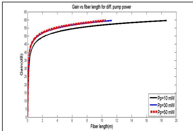
Figure (9): Gain vs. fiber length at diff. pump power of (YDFA), \lambda_p=968 nm, \lambda_s=1022 nm, a=2.5\mu\text{m} , N=3.5 \times 10^{25} ion/m 3 .
