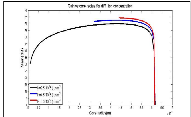
Figure (11): Gain vs core radius at diff. ion concentration of (YDFA), L=10 m, \lambda_p=968 nm, \lambda_s=1022 nm, p_p=25 mW.
