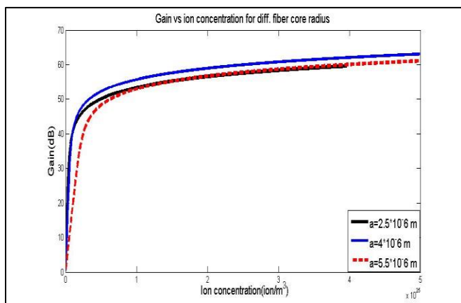
Figure (4): Gain vs. ion concentration at diff. core radius of (YDFA), L=10\text{m} , \lambda_p=968\text{nm} , \lambda_s=1022\text{nm} , p_p=25\text{ mW} .
