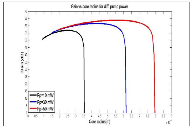
Figure (12): Gain vs. core radius at diff. pump power of (YDFA), L=10 m, \lambda_p=968 nm, \lambda_s=1022 nm, N=3.5 \times 10^{25} ion/m 3 .
