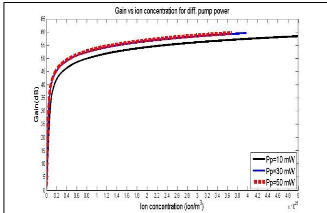
Figure(2): Gain vs. ion concentration at diff. pump power of (YDFA), L=10\text{m} , \lambda_p=968\text{nm} , \lambda_s=1022\text{nm} , a=2.5\mu\text{m} .
