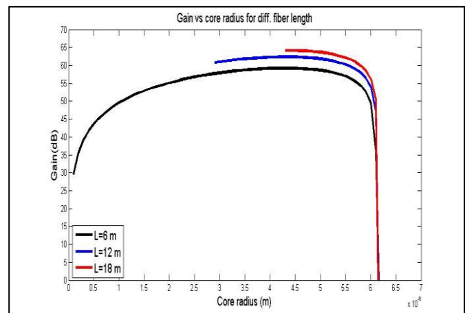
Figure (13): Gain vs. core radius at diff. fiber length of (YDFA), p_p=25 mW, \lambda_p=968 nm, \lambda_s=1022 nm, N=3.5 \times 10^{25} ion/m 3 .
