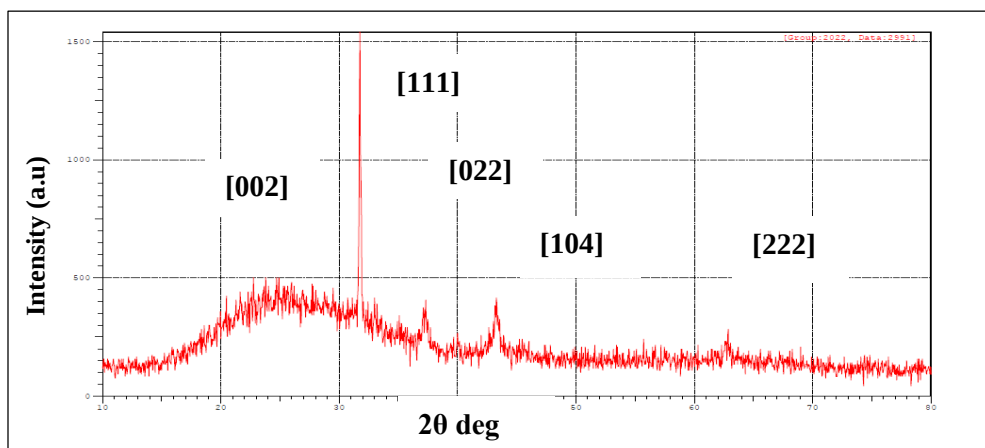
Fig(6): X- ray diffraction of \text{NiCl}_2:\text{Al}_2\text{O}_3 thin film (1%) at 350 °C.
