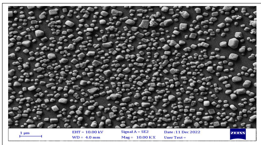
Fig(14): SEM image of \text{NiCl}_2:\text{Al}_2\text{O}_3 thin film (1%) at 350°C.
