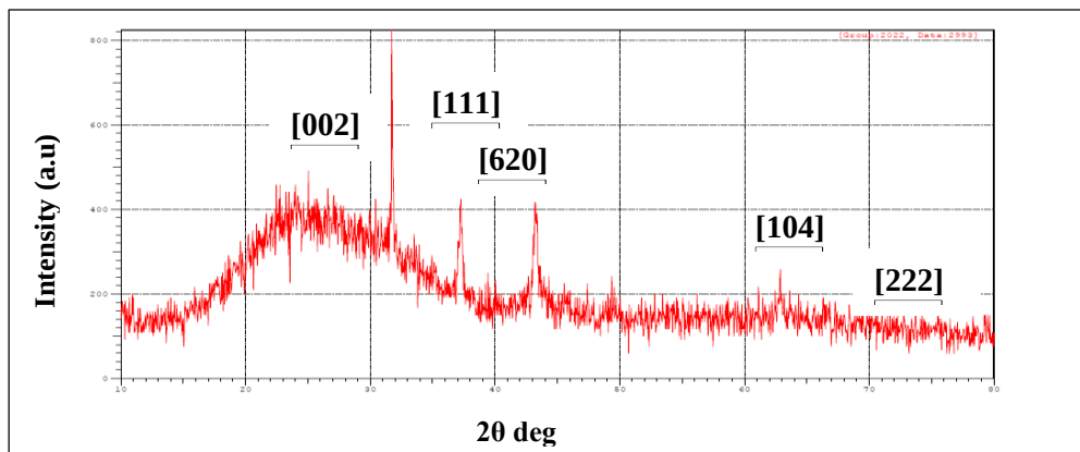
Fig(8): X- ray diffraction of \text{NiCl}_2:\text{Al}_2\text{O}_3 thin film (3%) at 350 °C.
