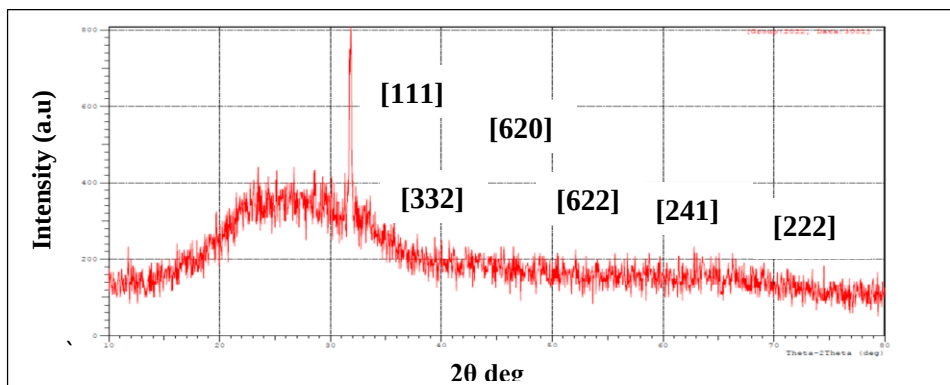
Fig(4): X-ray diffraction of \text{NiCl}_2:\text{Al}_2\text{O}_3 thin film at 3%.
