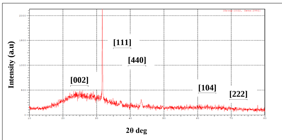
Fig(7): X- ray diffraction of \text{NiCl}_2:\text{Al}_2\text{O}_3 thin film (2%).
