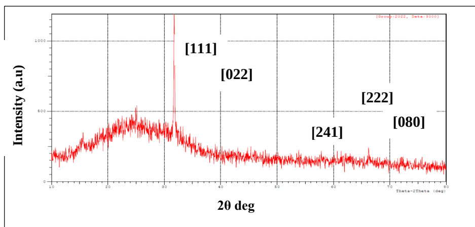
Fig(2): X-ray diffraction of \text{NiCl}_2:\text{Al}_2\text{O}_3 thin film at 1%.
