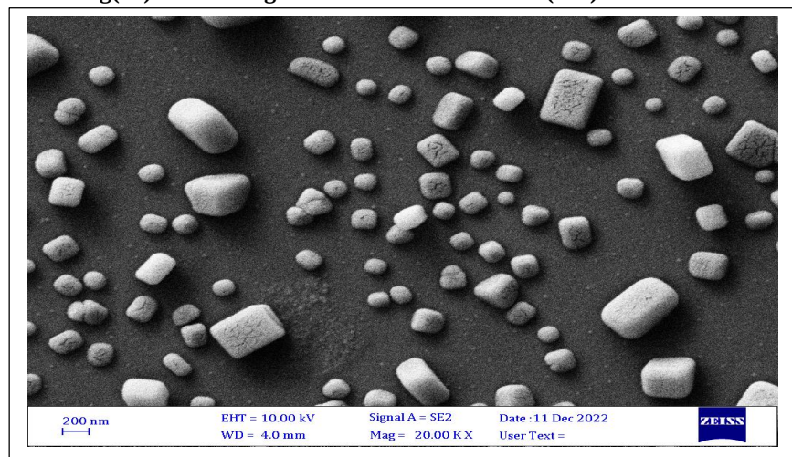
Fig(15): SEM image of \text{NiCl}_2:\text{Al}_2\text{O}_3 thin film (2%) at 350°C.
