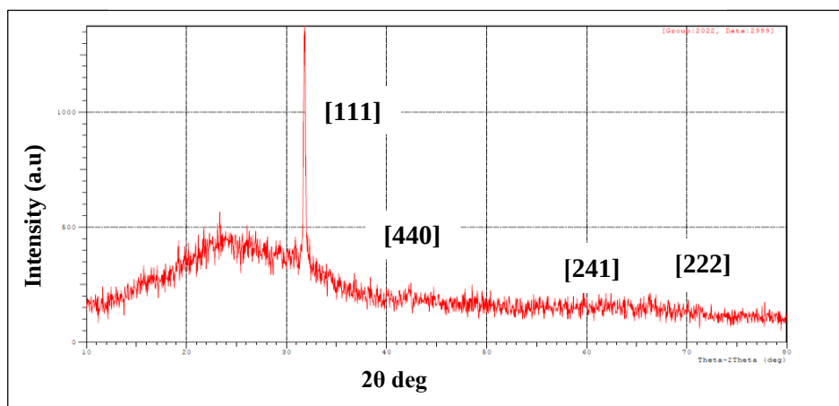
Fig(3): X-ray diffraction of \text{NiCl}_2:\text{Al}_2\text{O}_3 thin film at 2%.
