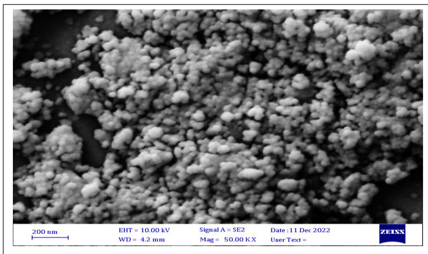
Fig(16): SEM image of \text{NiCl}_2:\text{Al}_2\text{O}_3 thin film (3%) at 350^\circ\text{C} .
