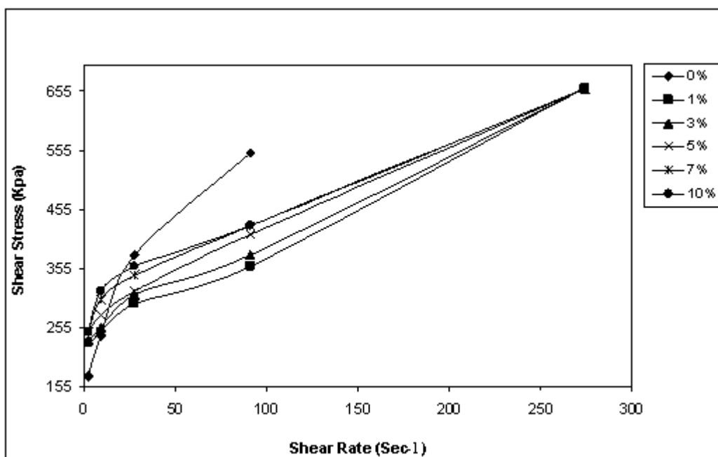
Fig. 3. Relationship between apparent shear stress and shear rate for PE/asphalt and 1% peroxide at 210 °C
