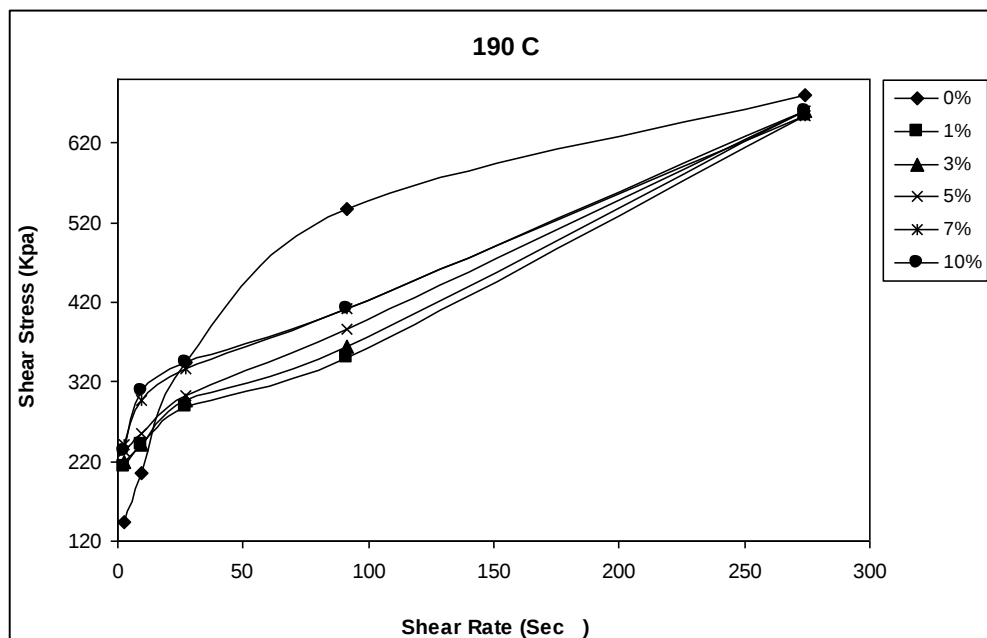
Fig. 2. Relationship between apparent shear stress and shear rate for PE/asphalt and 1% peroxide at 190 °C
