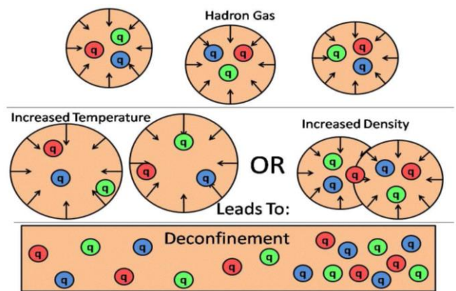
Figure 3: Deconfinement representation [5].
