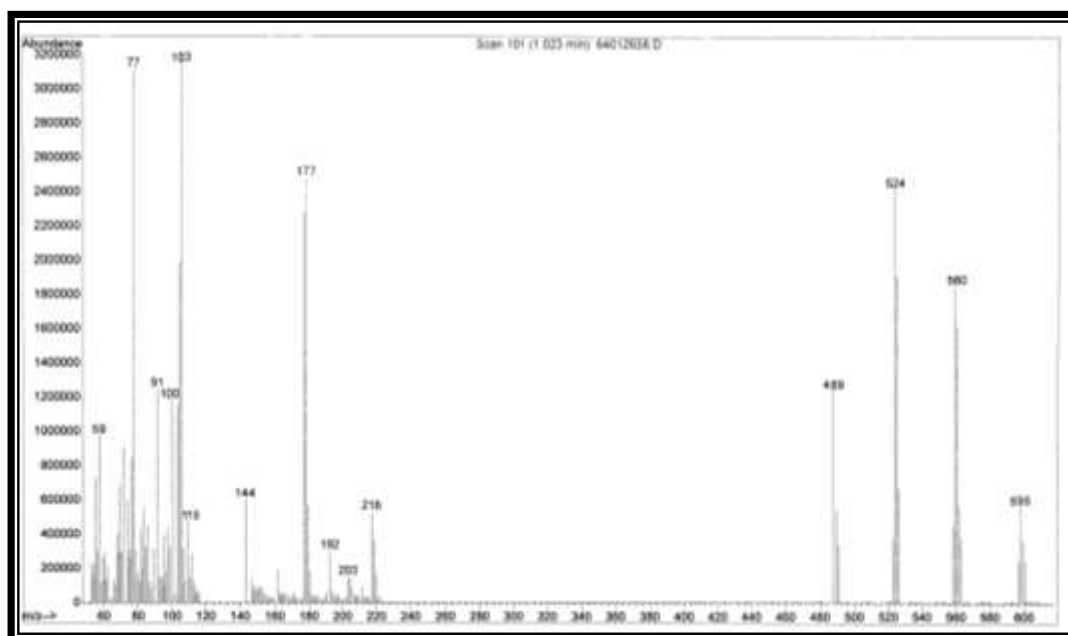
Figure (9) mass spectrum of [\text{Cr}(\text{L})_2\text{Cl}_2]\text{Cl}
