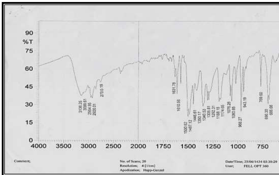
Figure(4) IR spectrum of Ligand ( C_{10}H_{10}N_4S )
