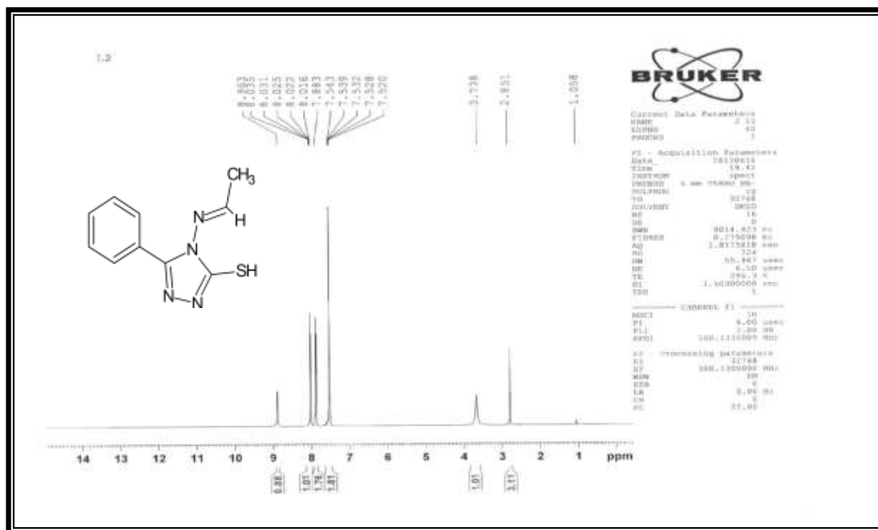
Figure(7) ^1\text{H} NMR spectrum of the ligand ( \text{C}_{10}\text{H}_{10}\text{N}_4\text{S} )
