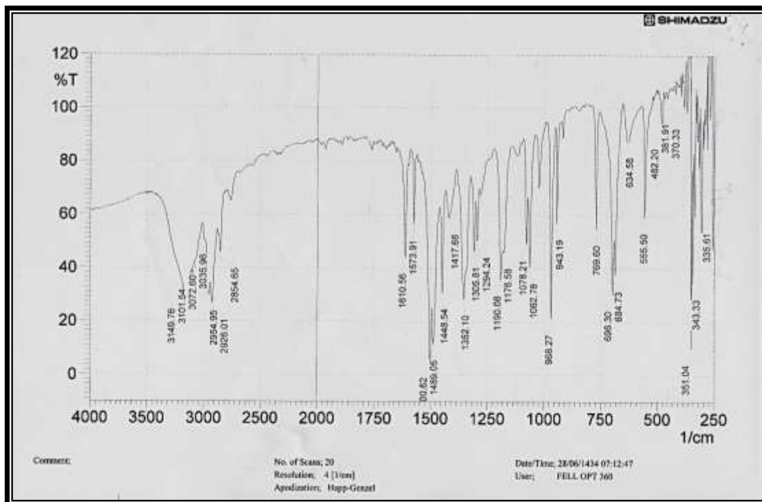
Figure(6) IR spectrum of [\text{Ni}(\text{L}) \text{Cl}_2]
