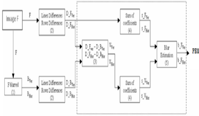
Figure (2): Flow chart of the PBM algorithm [9].
