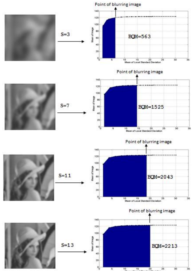
Figure (5): The BQM for blurring lena images at different values of sigma, these value direct proportional with the area under the curve in the ( m, g ) mode after they reblurring at ( S=3,7,11,13 ).
