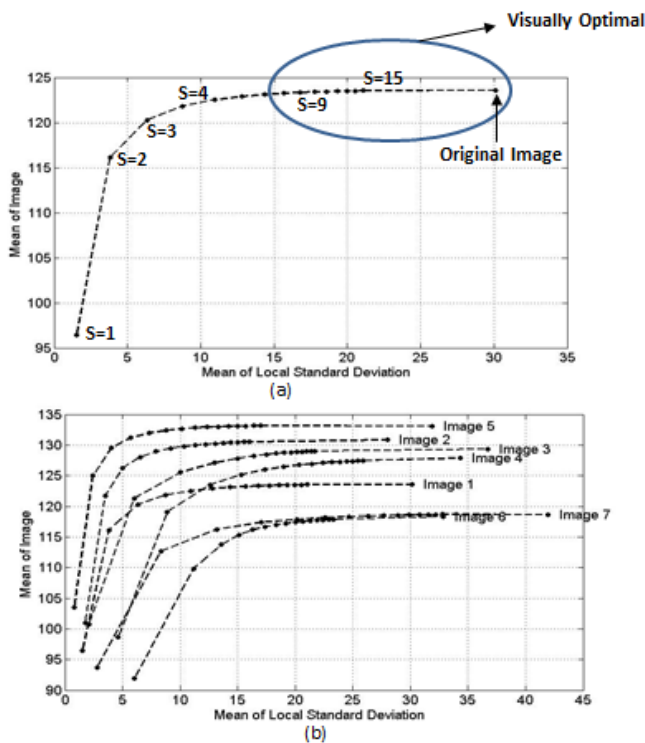
Figure(4): The MLSD model in (a) the original (Lena) image and Gaussian blurring of this image with different value of s ( from 1 to 15) and (b) same model for data images.
