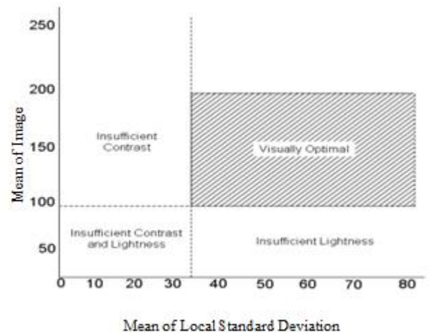
Figure (3): Image quality description according to MLSD model [11].
